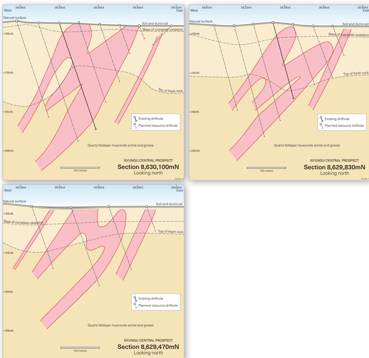
Figure 4 Nyungu Central cross sections showing existing and planned drill holes.
