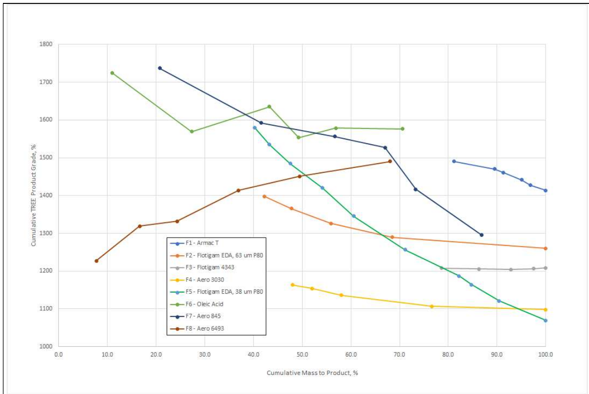
Figure 3.1 : Cumulative TREE Product Recovery-Grade Curves
