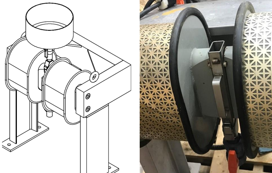
Figure 3 Eriez Magnetic Separator for Wet Mag-separation
