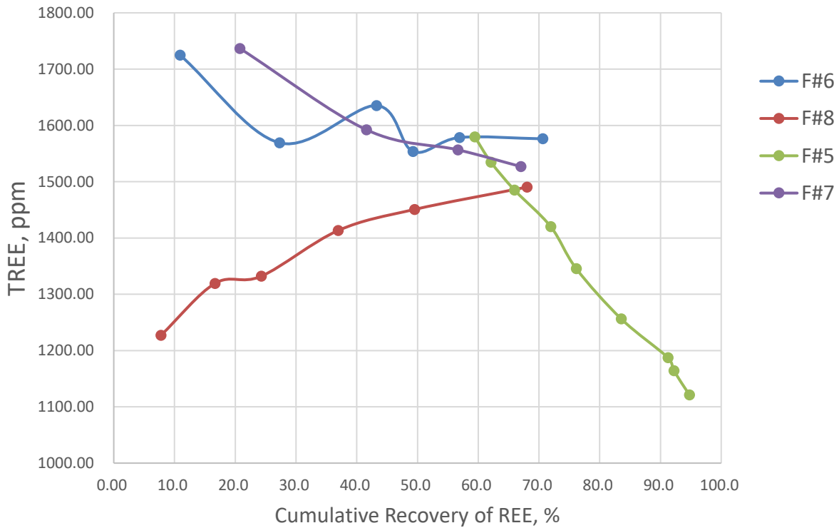
Figure 4 A Summary of Preliminary Flotation F#5-F#8
