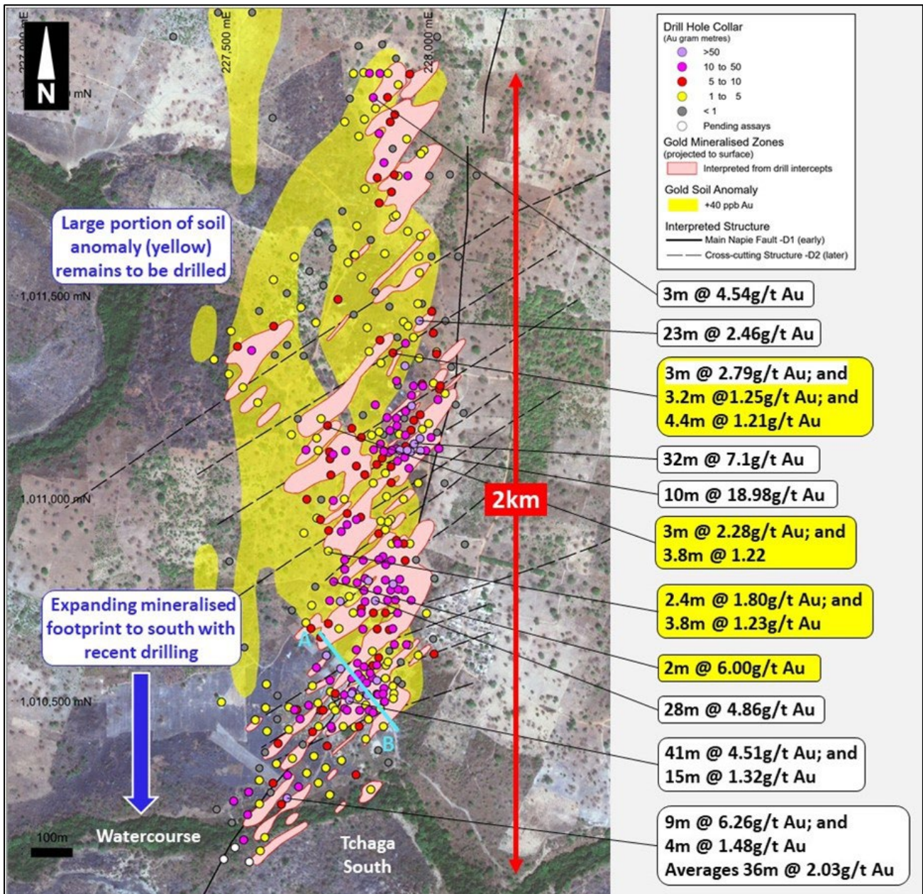
Figure 5: Tchaga Prospect - Select previous (white) and current (yellow) gold intercepts – note the abundance of purple (>50 gram metre) and pink (10-50 gram metre) drill intercepts and the +40ppb gold soil geochem anomaly shaded yellow which highlights future drill targets to extend known mineralisation
