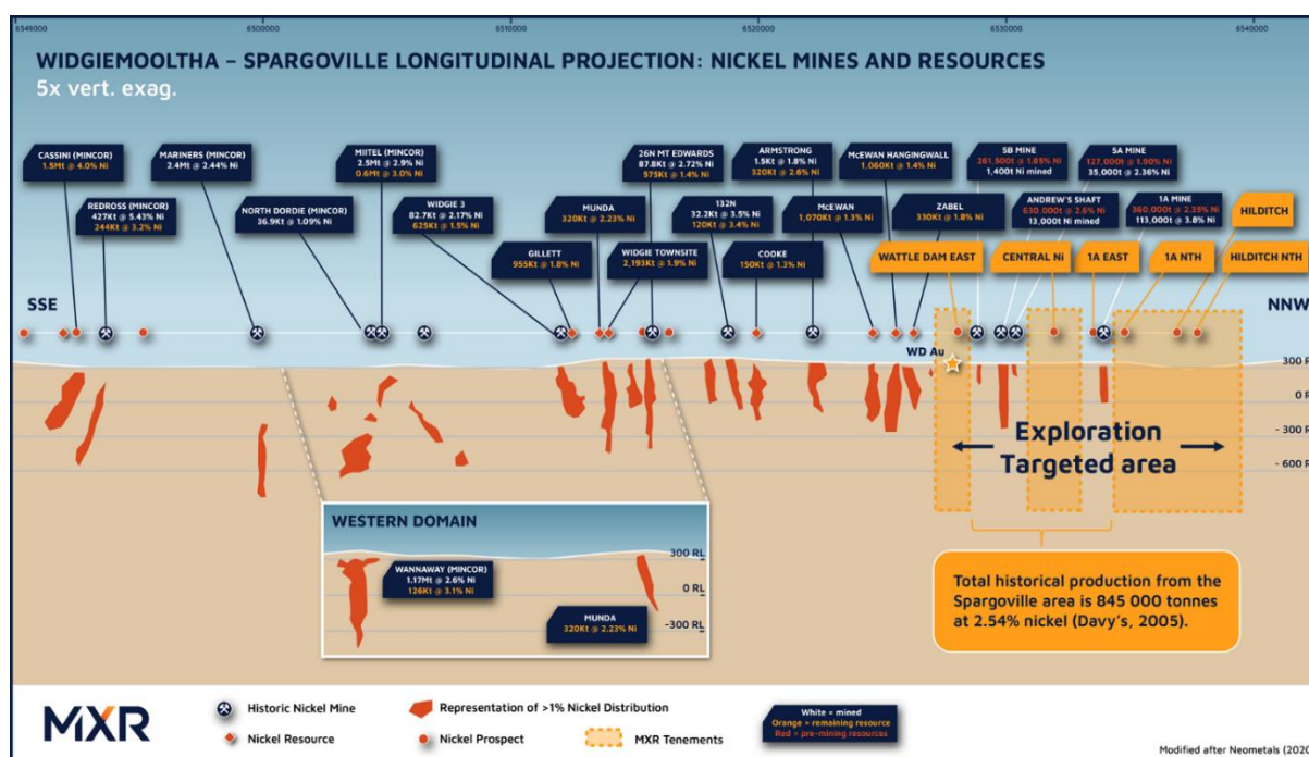
Figure 1. Longitudinal projection of the nickel deposits and mines in the Widgiemoooltha – Hilditch belt, looking west. Orange polygons at right of image indicate where Maximus Resources holds key tenements over the prospective trend.
