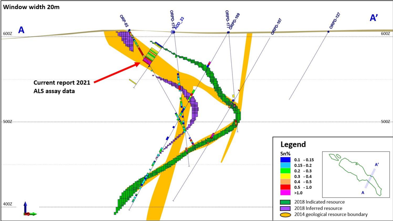
Figure 2. Oropesa 2021 resource infill diamond drilling, ADD_23
