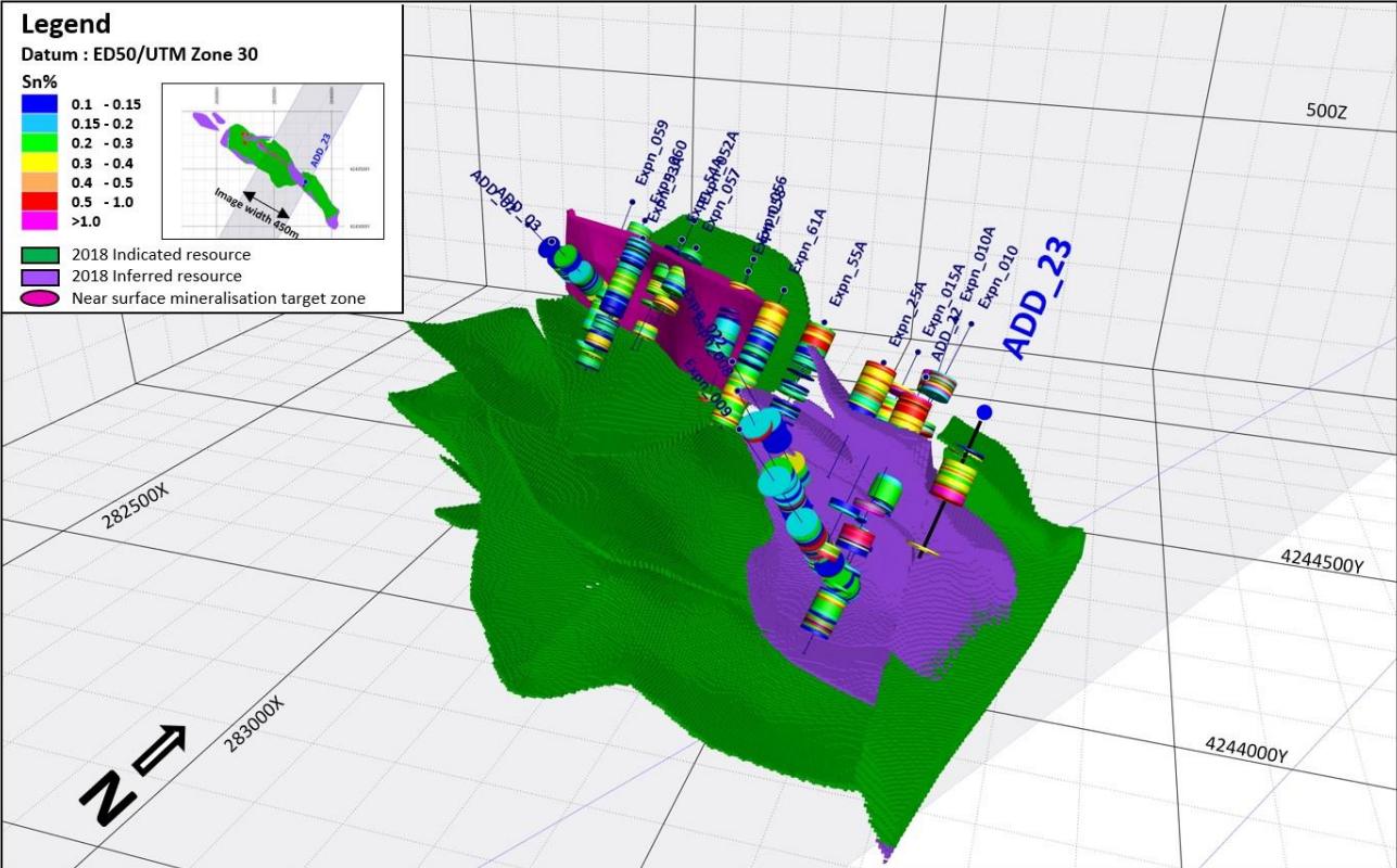
Figure 4. Detailed 3D image of the location of mineralisation intersected in ADD_23, with additional information from shallow drill holes from the recently completed diamond drilling program depicting confirmation and continuity of the shallow mineralisation target.
