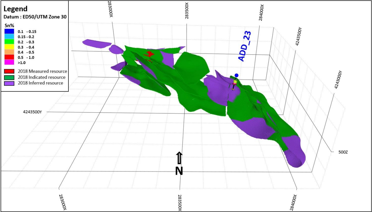
Figure 3. Oropesa 3D image of 2018 geological resource depicting the location of ADD_23
