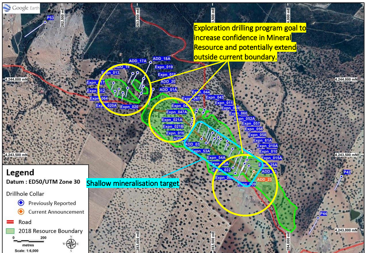
Figure 1. Location of drill holes with reported assay data as at 28 th September 2021, from the exploration drilling program at the Oropesa Tin Project, Spain
