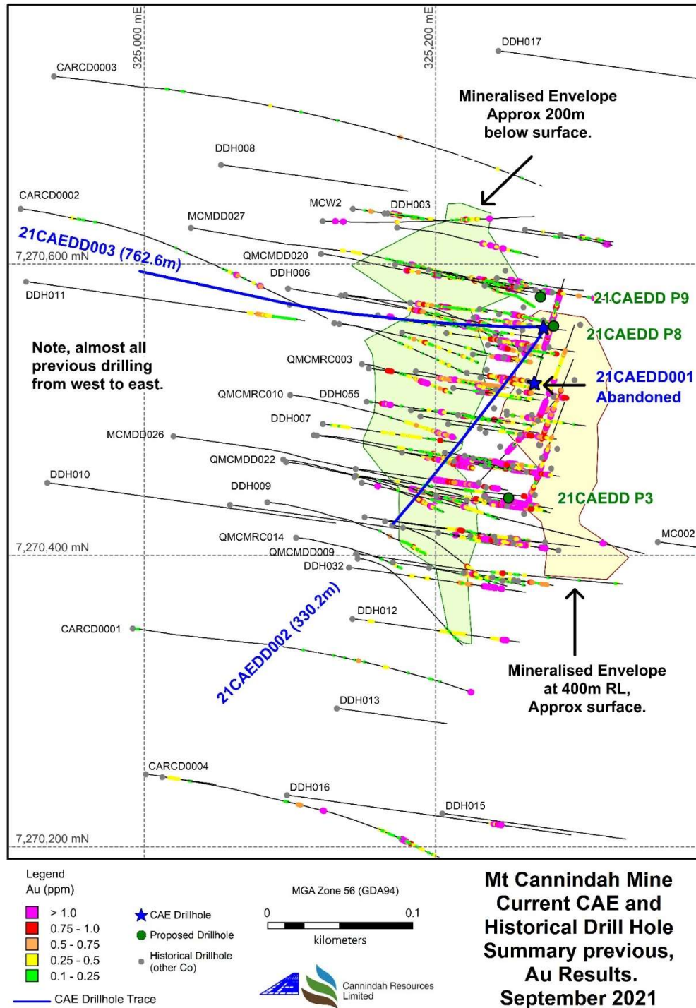
Fig 5. Mt Cannindah mine area ,plan view of recent drillhole 21CAEDD002 & 3 traces in relation to previous drilling and gold results. Also shown are the mineralised envelopes at surface (400m RL) and 200m below surface. These envelopes are mainly defined by >0.3 % Cu, they contain the current resource block model.
