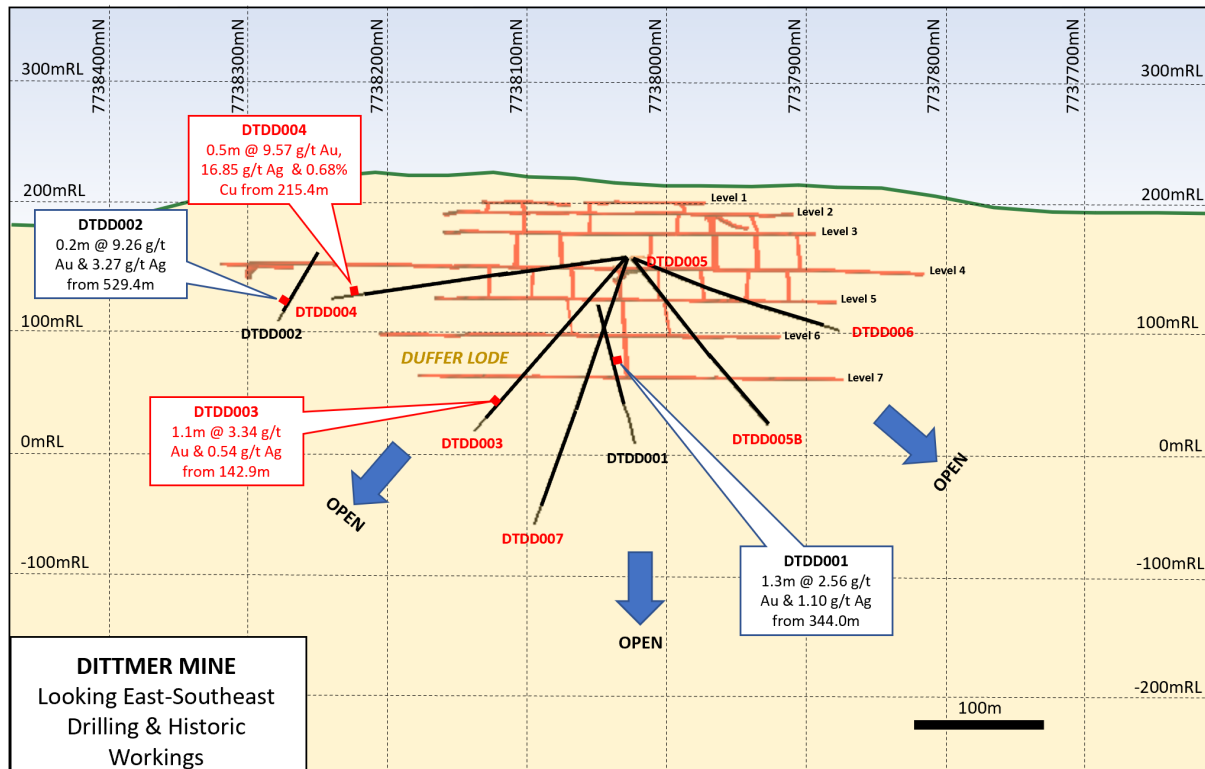
Figure 2. Dittmer Drilling
