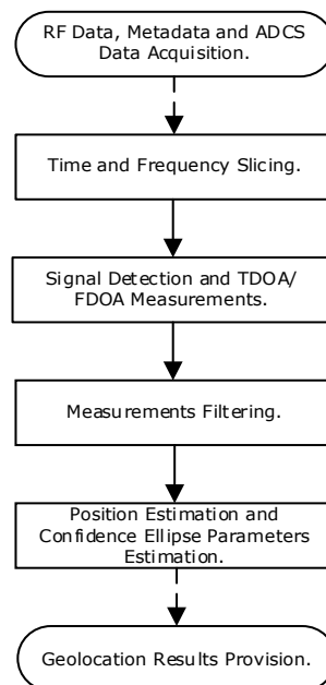
Figure 2 – Geolocation System software flowchart.
