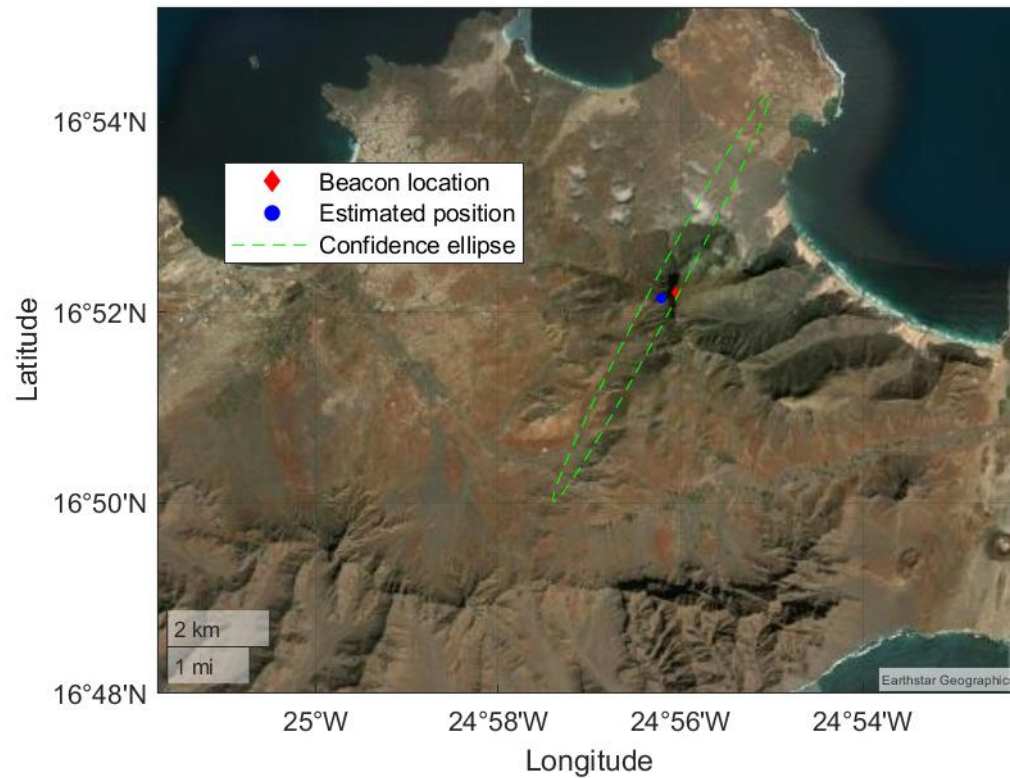
Figure 6 - Confidence ellipse of the position estimate.
