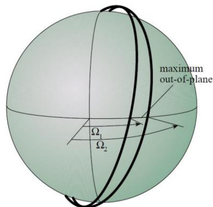
Figure 8 – Cluster Orbit Representation.
