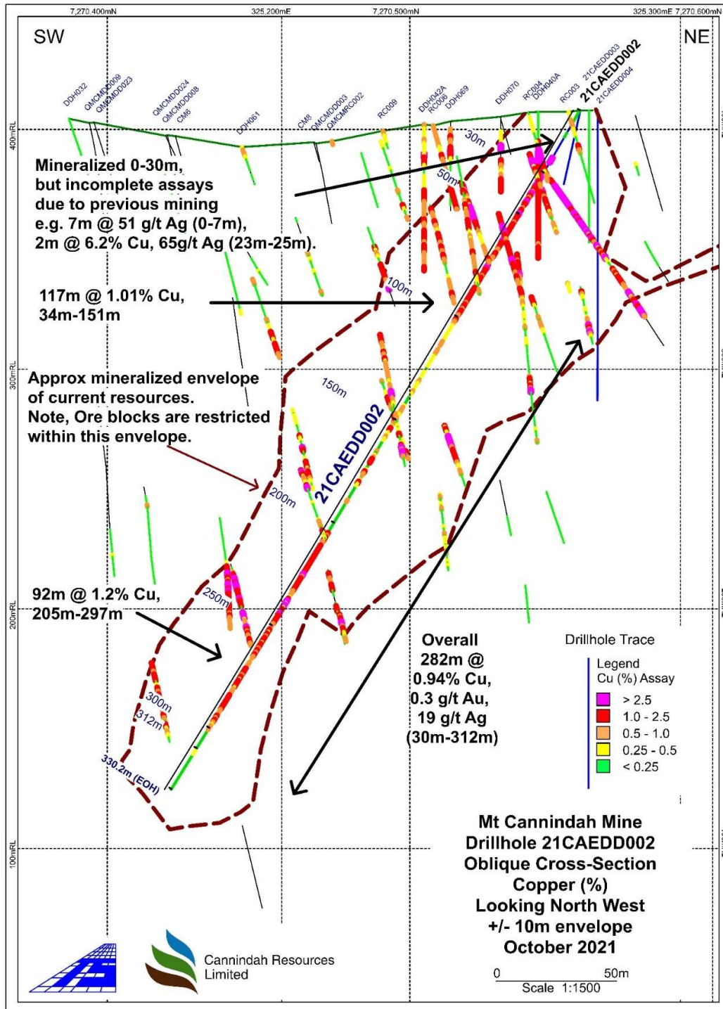
Fig 5. Mt Cannindah cross section (20m window) showing trace of hole 21CAEDD002 with complete assay results. Also shown are historic copper intercepts and mineralized envelope containing the blocks within the current resource model.
