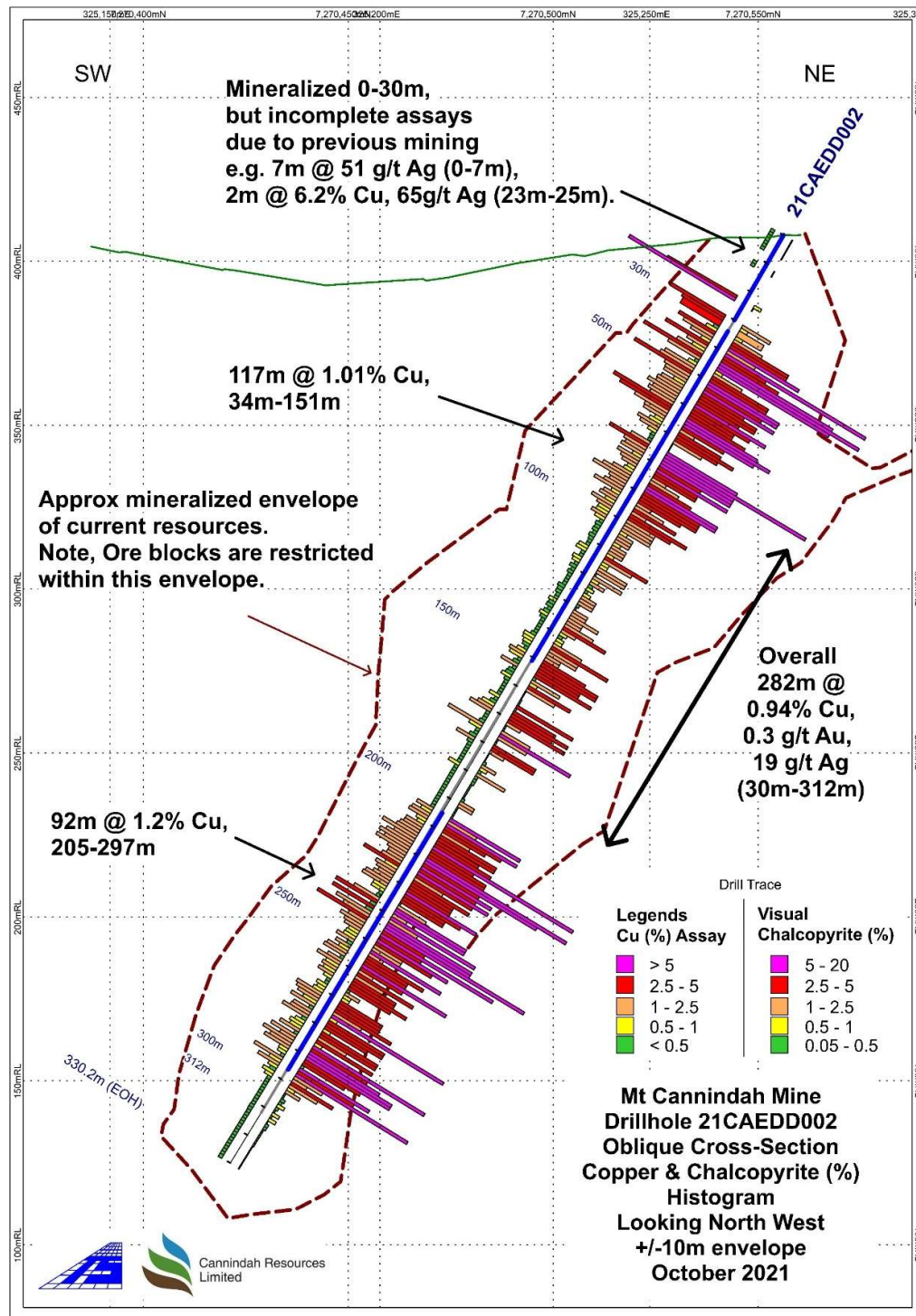
Fig 6. Mt Cannindah cross section profile hole 21CAEDD002 with histogram of copper lab assay results for complete hole, plotted against visual estimates chalcopyrite content.
