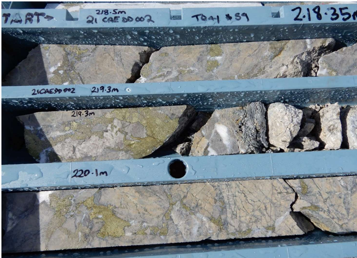
Fig 8. Primary copper mineralisation Hole 21CAEDD002 , 219,220m ,8%-10% visual estimate of chalcopyrite in the interval 219m-221m. Lab assay result 2.00% Cu
