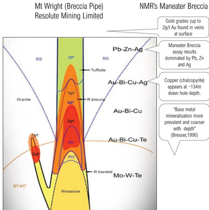
Figure 8: Schematic diagram from Resolute Mining's Mt Wright Breccia Pipe showing the metal zoning observed in association with gold mineralisation at depth. A review of existing data contained within publicly accessible reports from previous explorers shows similarities with the zoning observed at the Mt Wright Breccia including a zone of high lead, zinc, and silver, but low gold near the top of the breccia and above the zone of primary gold mineralisation. Features found at the Maneater Breccia are listed on the right-hand side of the cross section. The schematic section through the Mt Wright Breccia Pipe obtained from a Resolute Mining Limited Presentation (2013). The upper part of the metal zoning is analogous to the results from the single drill hole in the Maneater Breccia on EPM 28038.
