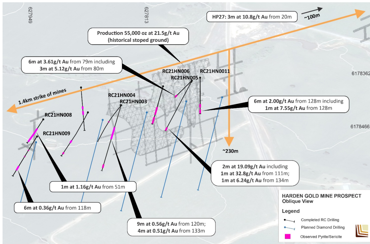
Figure 4: Oblique view of drilling at the Harden Gold Mine Prospect Looking South-West
