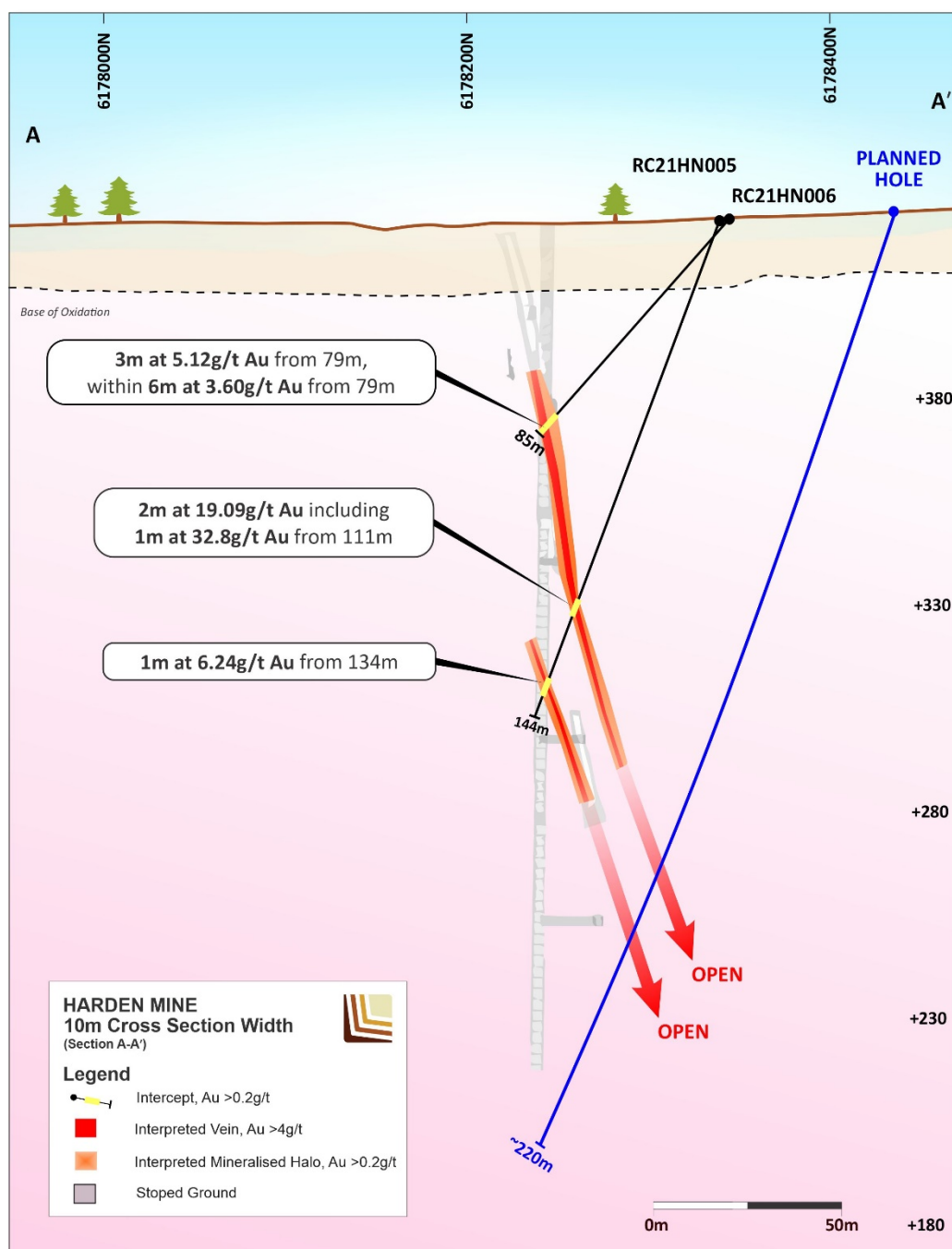
Figure 1: Cross Section showing interpreted veins and mineralised halo (0.2g/t Au cut-off grade)
