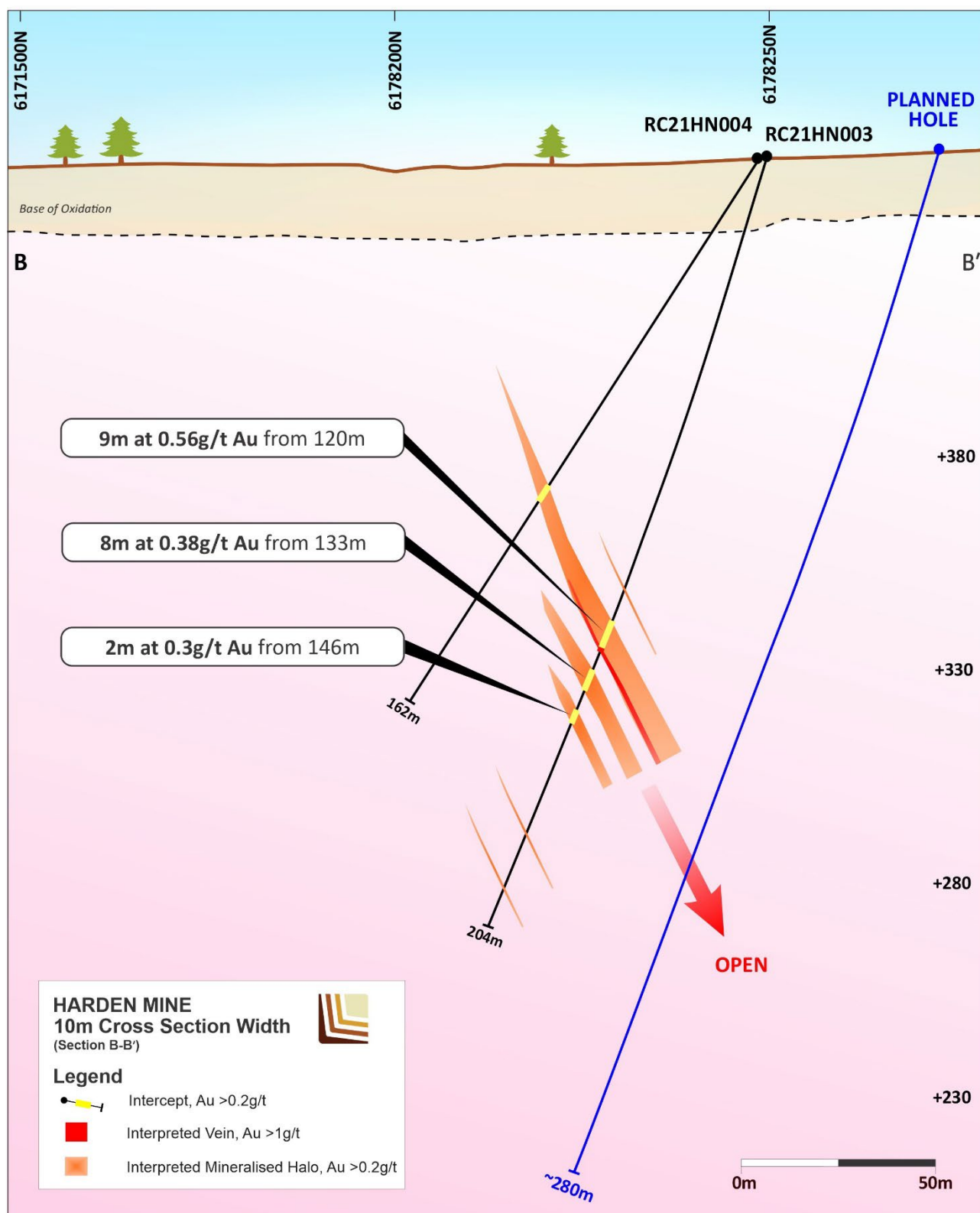
Figure 2: Cross Section showing interpreted veins and mineralised halo (0.2g/t Au cut-off grade)
