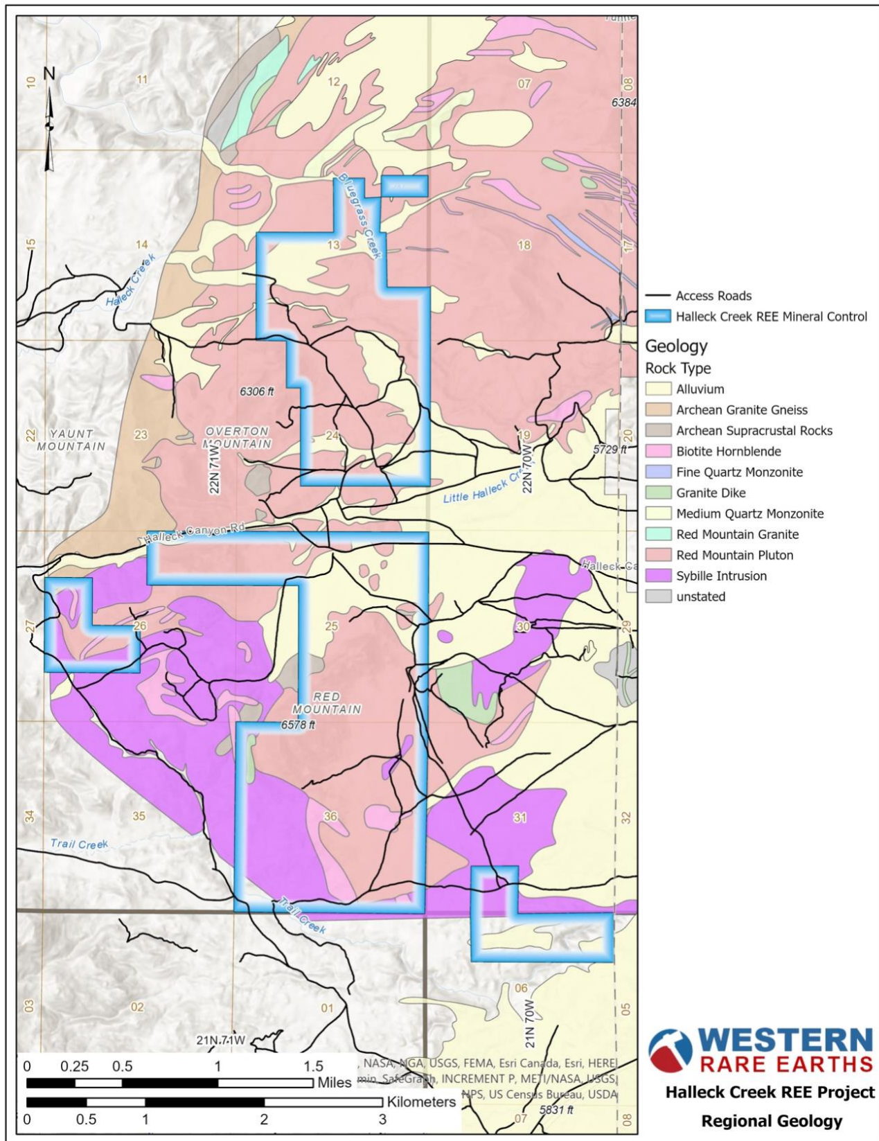
Regional Geology
