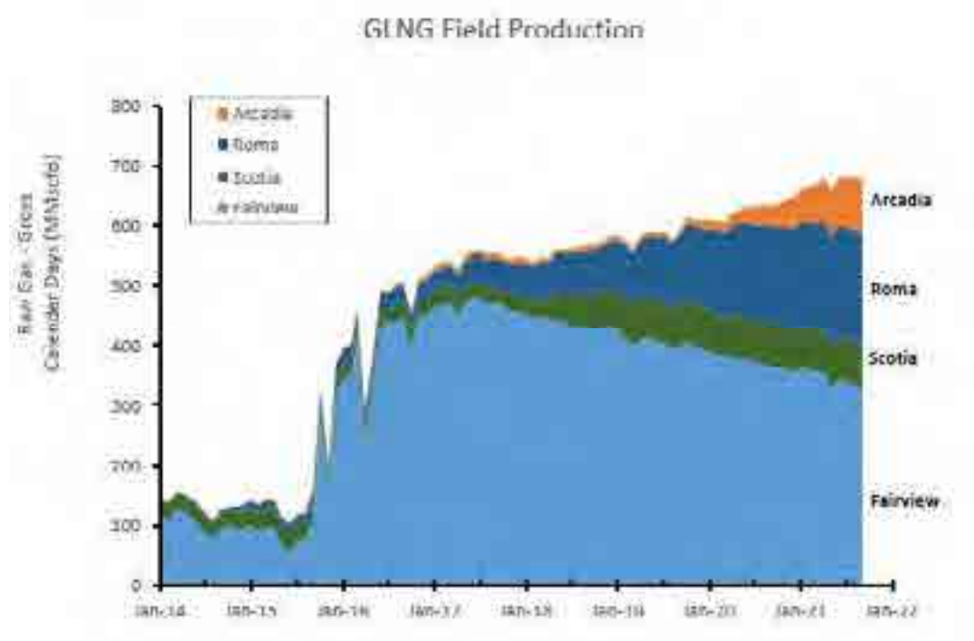
Figure 5.62: GLNG Project Historical Performance
