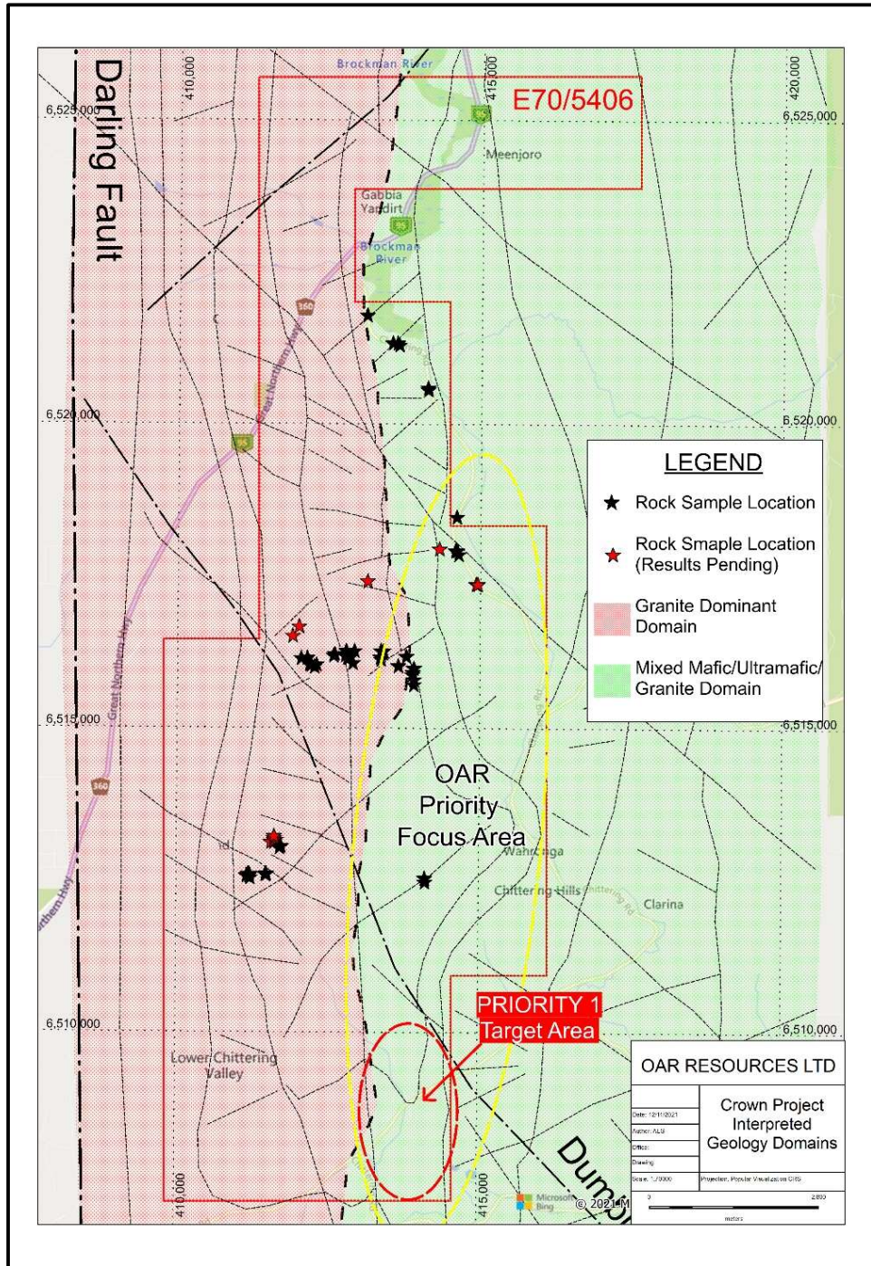
Figure 2: Crown Project - Interpreted broad lithological domains
