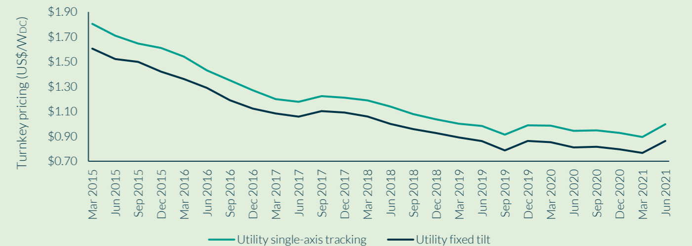
Figure 3: Cost of Solar
