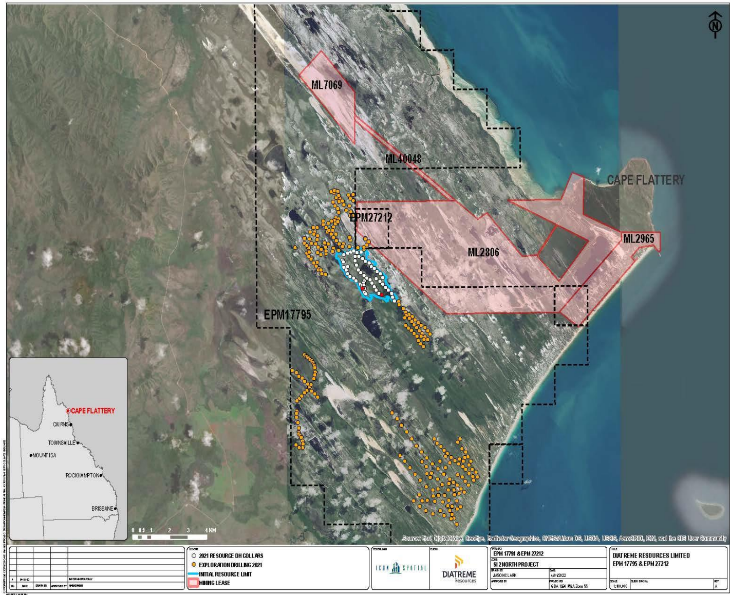
Fig 2 – Si 2 North Project - Resource Area and Regional Exploration
