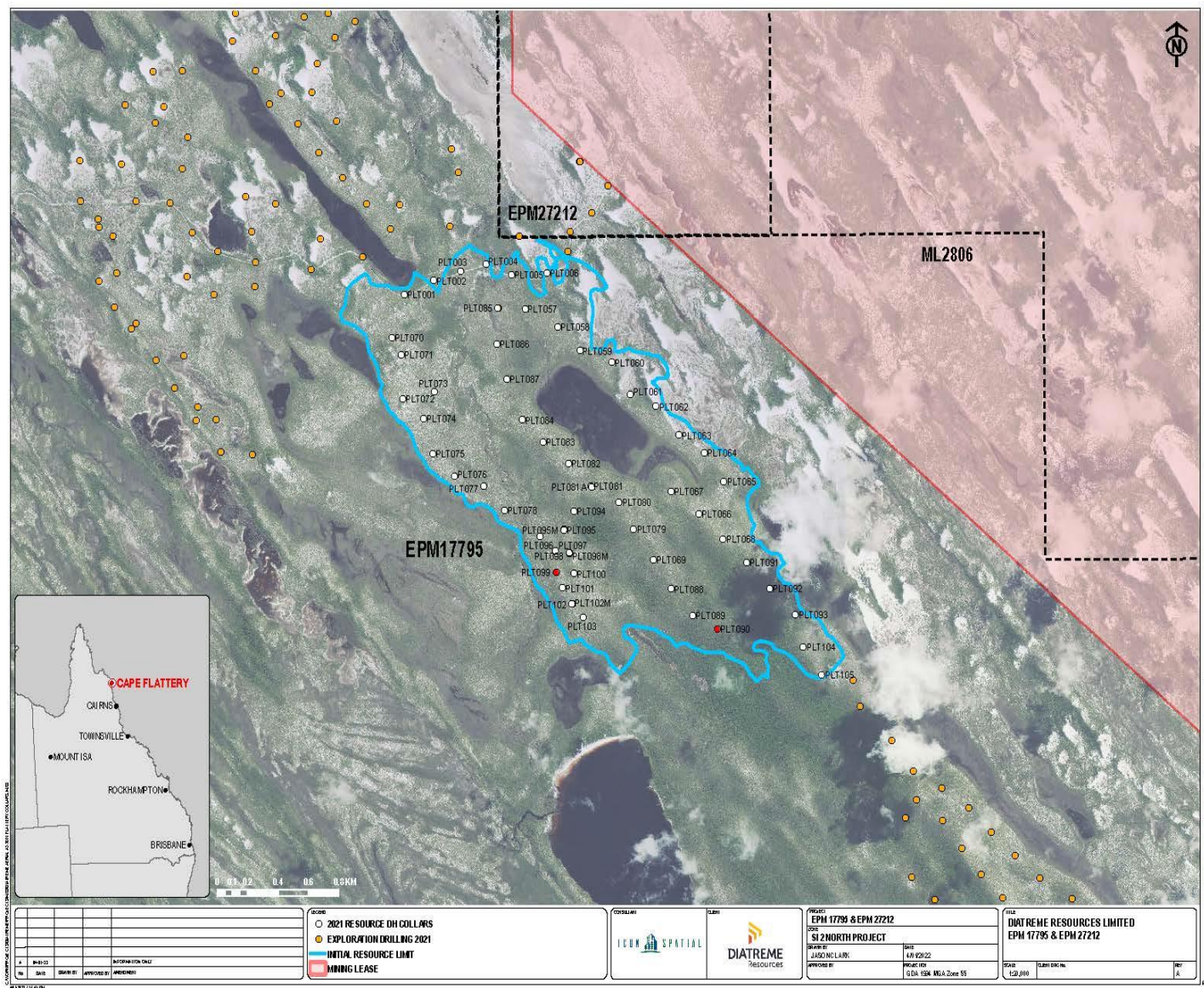
Fig 1 – Si 2 North Project – Resource Area and Drill Holes
