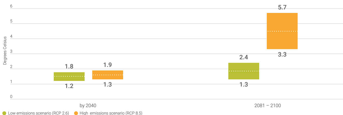
CHART 6: POTENTIAL FUTURE TEMPERATURE INCREASES UNDER THESE SCENARIOS
