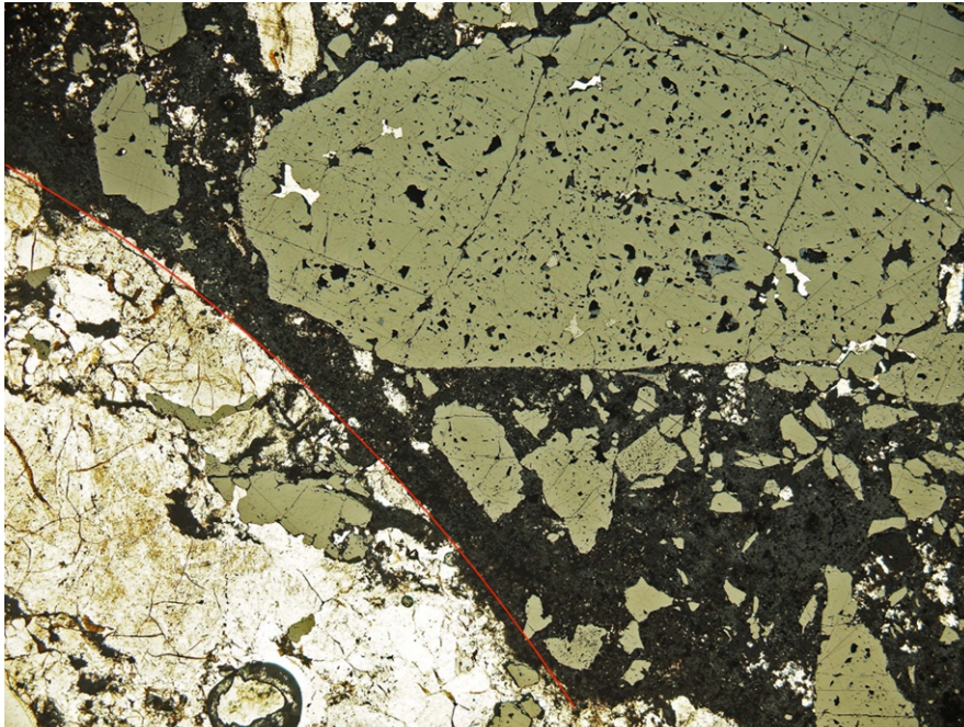
Figure 5: Photo-micrograph of PPRC826 152-153m sample illustrating multi-stage character of the mineralised hydrothermal vein with early quartz+pyrite vein (bottom left below red line) cross cut by a later vein (upper side of red line) composed of large angular pyrite fragments (dark yellow) containing small native silver grains within a fine grained dark cement composed of quartz, pyrite and hematite/?goethite (scale – top to bottom of image approximately 3mm).
