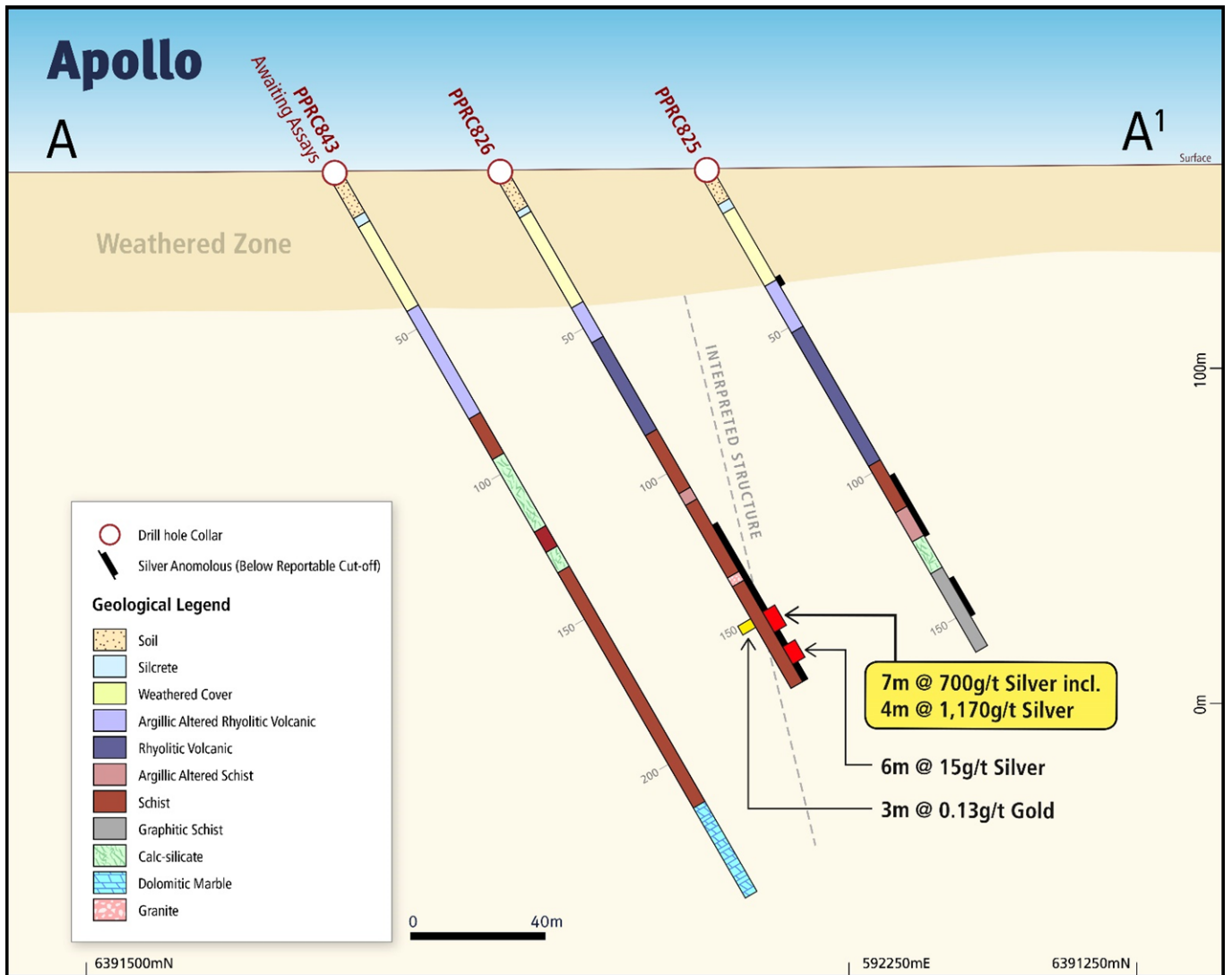
Figure 4: Apollo section showing significant intersections for first two holes drilled. Third hole awaiting results. Diamond hole will twin RC hole PPRC826.
