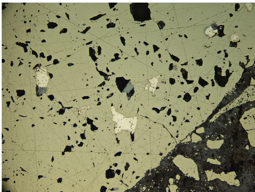
Figure 4: Photo-micrograph of PPRC826 152-153m sample showing angular grains of native silver (bright yellow) as inclusions within a larger (darker yellow) pyrite grain (scale – top to bottom of image approximately 0.7mm).
