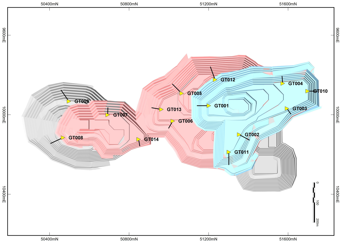
Figure 6: Diamond drill hole locations at Paris for geotechnical assessment.
