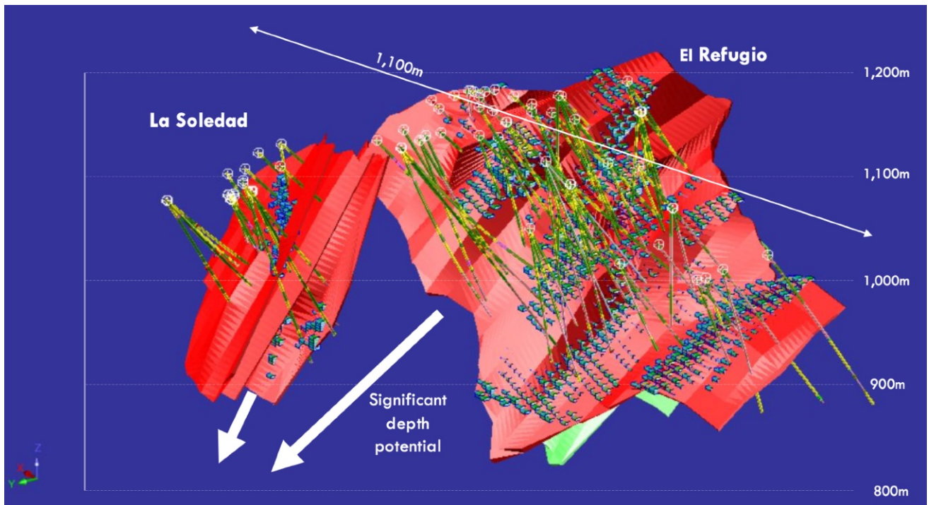
Figure 4 Oblique long section showing the La Soledad and El Refugio vein models with drill hole traces and resource block model Scale and elevations are approximate
