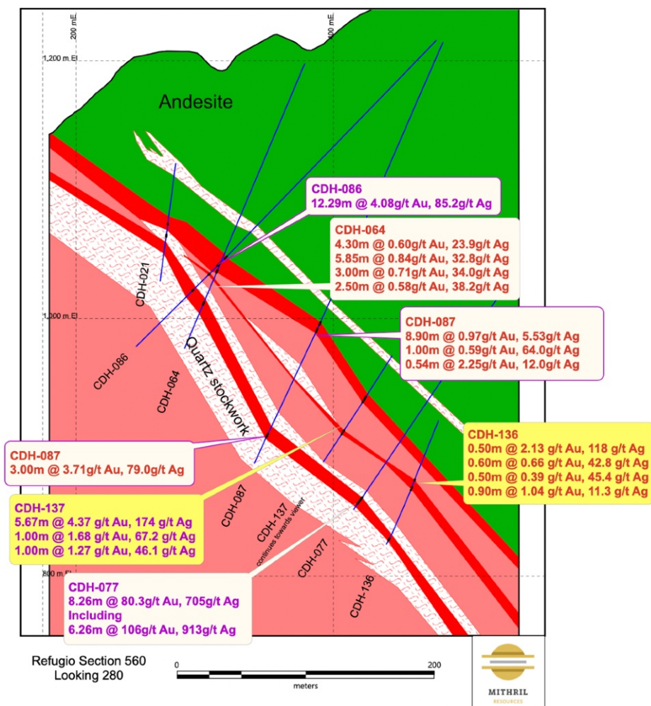
Figure 3 – Cross section on the western side of the El Refugio upwelling zone where deeper gold and silver mineralisation and geological observations confirm the considerable depth potential of the El Refugio hydrothermal system.
