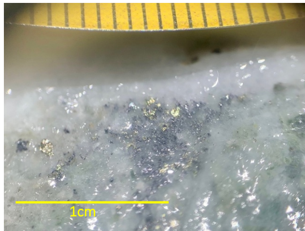
Figure 2 Photo of drill core from drill hole CDH-144 at 268m, showing black silver sulphides and sulphosalts and pyrite
