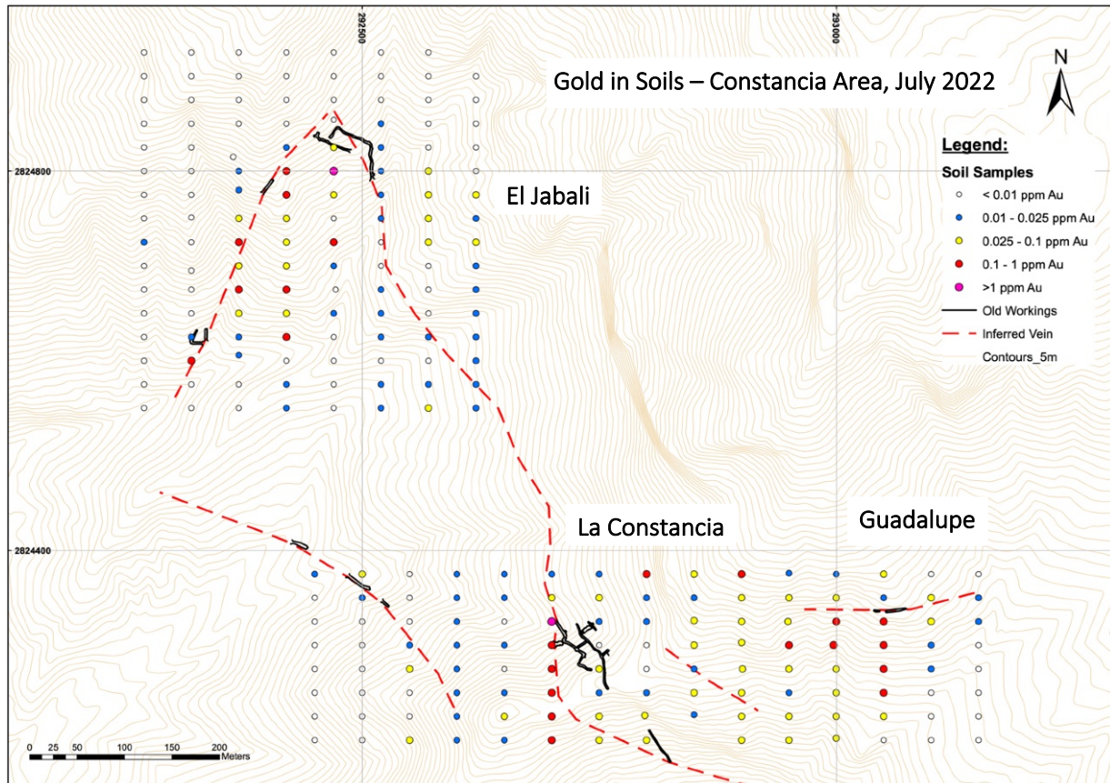
Figure 6 Gold in soils sampling map for the La Constanca area at the eastern end of the Copalquin District Middle Section, see Figure 1 for location
