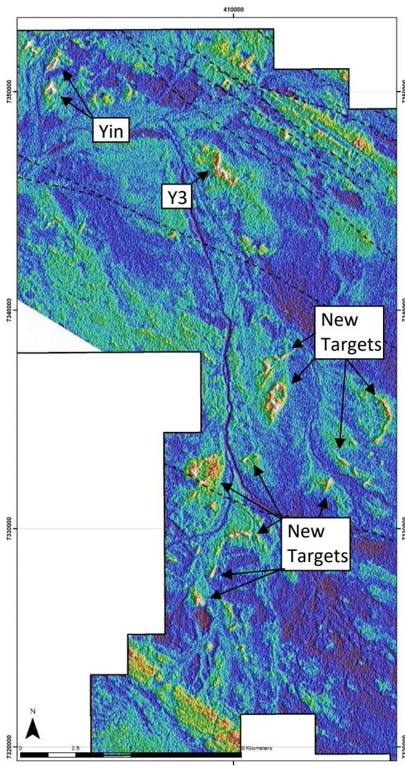
Figure 5: Image of a portion of the Thorium radiometric image showing the location of Yin, Y3 and some of the new targets to be assessed.
