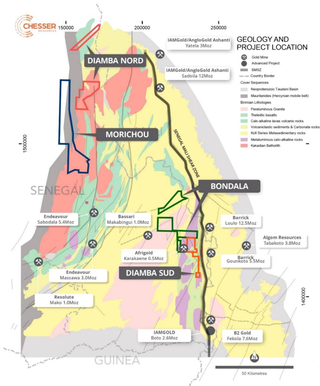
Figure 1: Schematic regional geology of eastern Senegal, showing Chesser's Project locations including the Diamba Sud Gold Project and its proximity to both the SMSZ and the major gold operations and projects.
