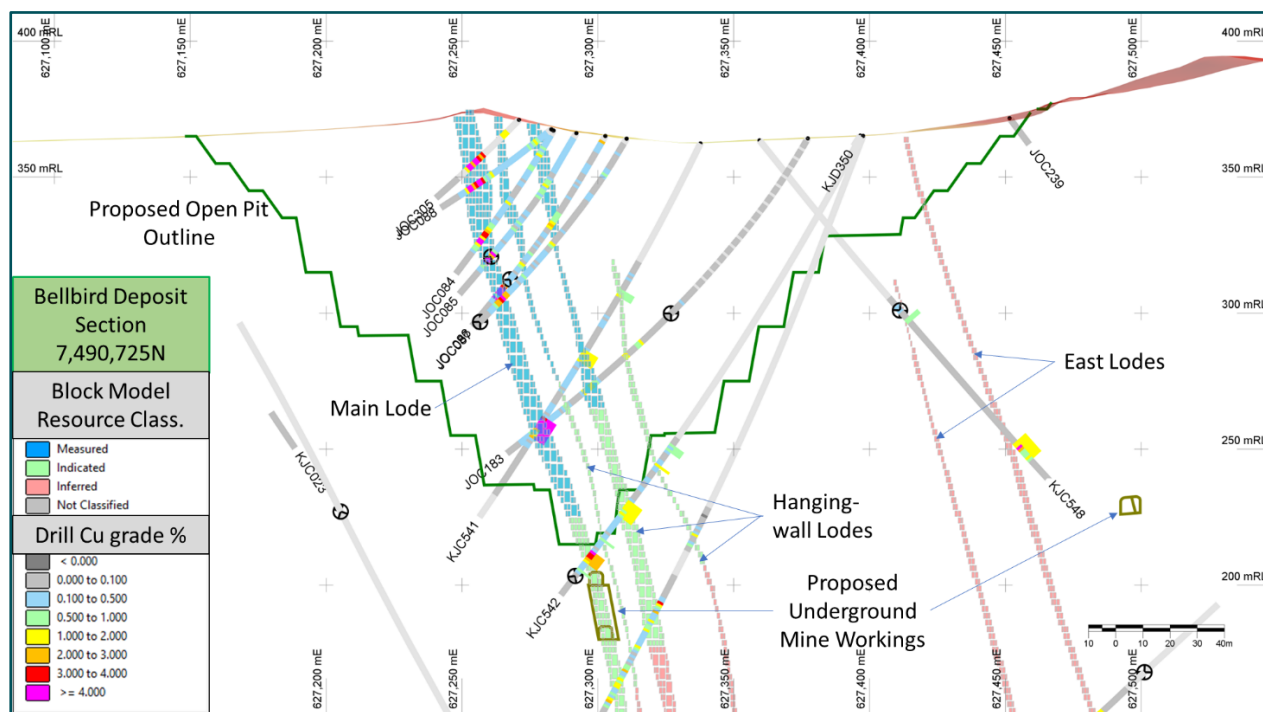
Figure 4: East-west cross section 7,490,725N through the proposed Bellbird open pit showing the new resource block model and drilling. The block model is coloured according to classification with blue blocks being Measured Resources, Green: Indicated Resources and Red: Inferred Resources. Drillhole traces are coloured by copper grade. New holes on this section are KJC541, KJC542 and KJC548.
