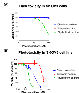
Figure 6. (A) Dark toxicity (without light activation) and (B) phototoxicity (exposure to red light of 660 nm) of Phyllochlorin sodium, Chlorin e4 sodium and Talaporfin sodium in SKOV3 ovarian cancer cells was assessed using AlamarBlue assay. Viability was expressed as % of untreated controls. n=4.
