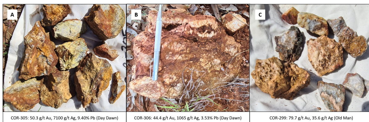
Figure 3 – Examples of rock chip samples from the Day Dawn – Old Man area.
