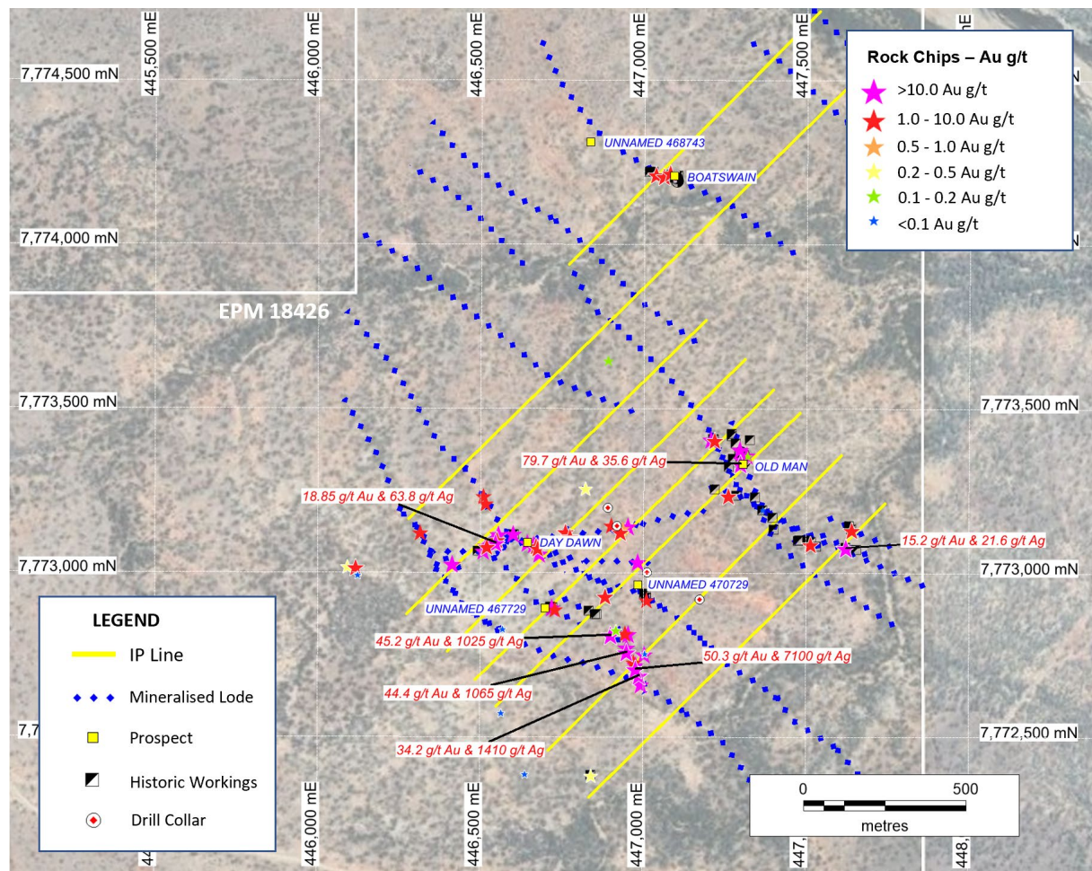
Figure 2 – Location of rock chip samples collected by Ballymore Resources from the Day Dawn – Old Man area.
