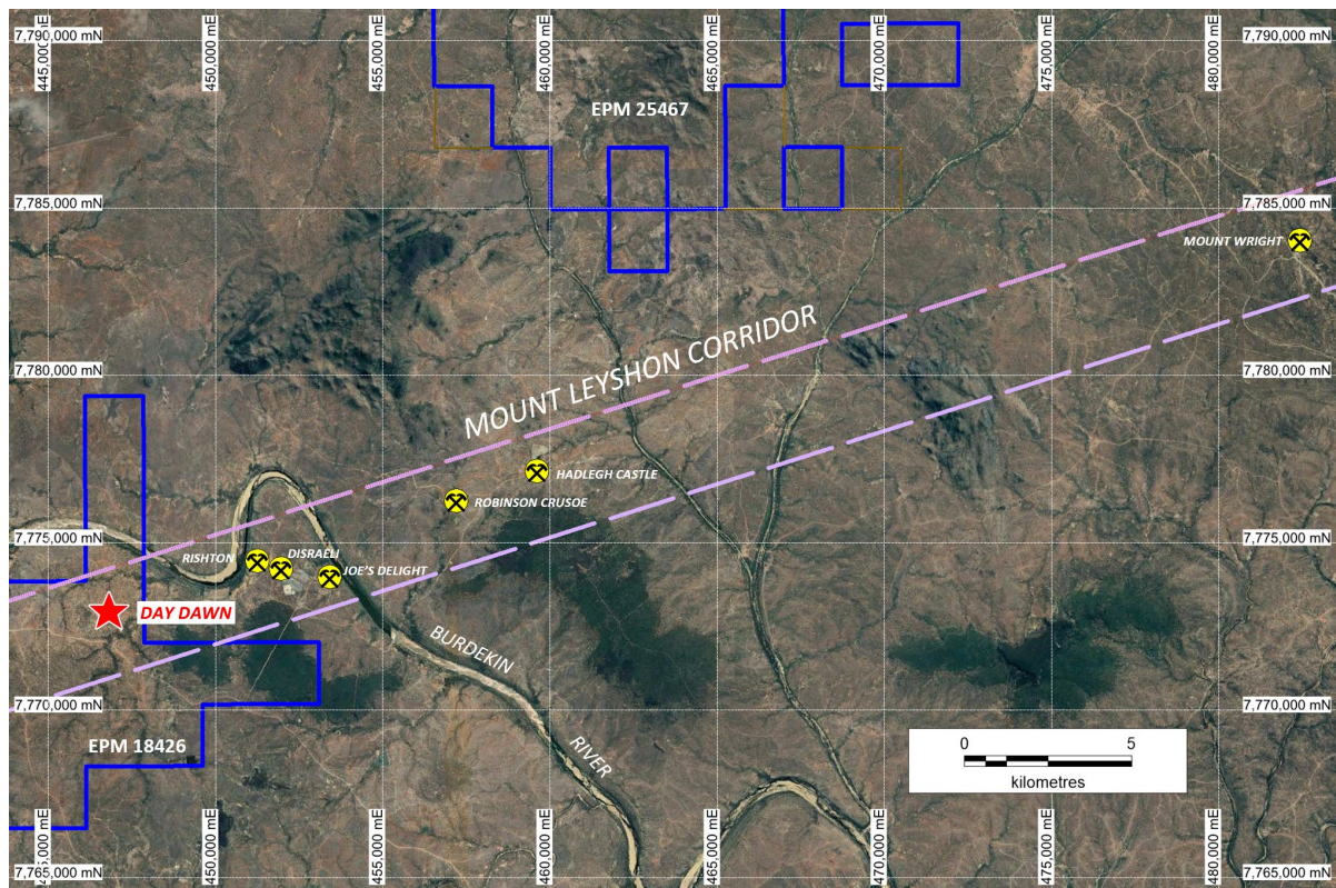
Figure 5 - Location of Day Dawn Prospect within Mount Leyshon Corridor
