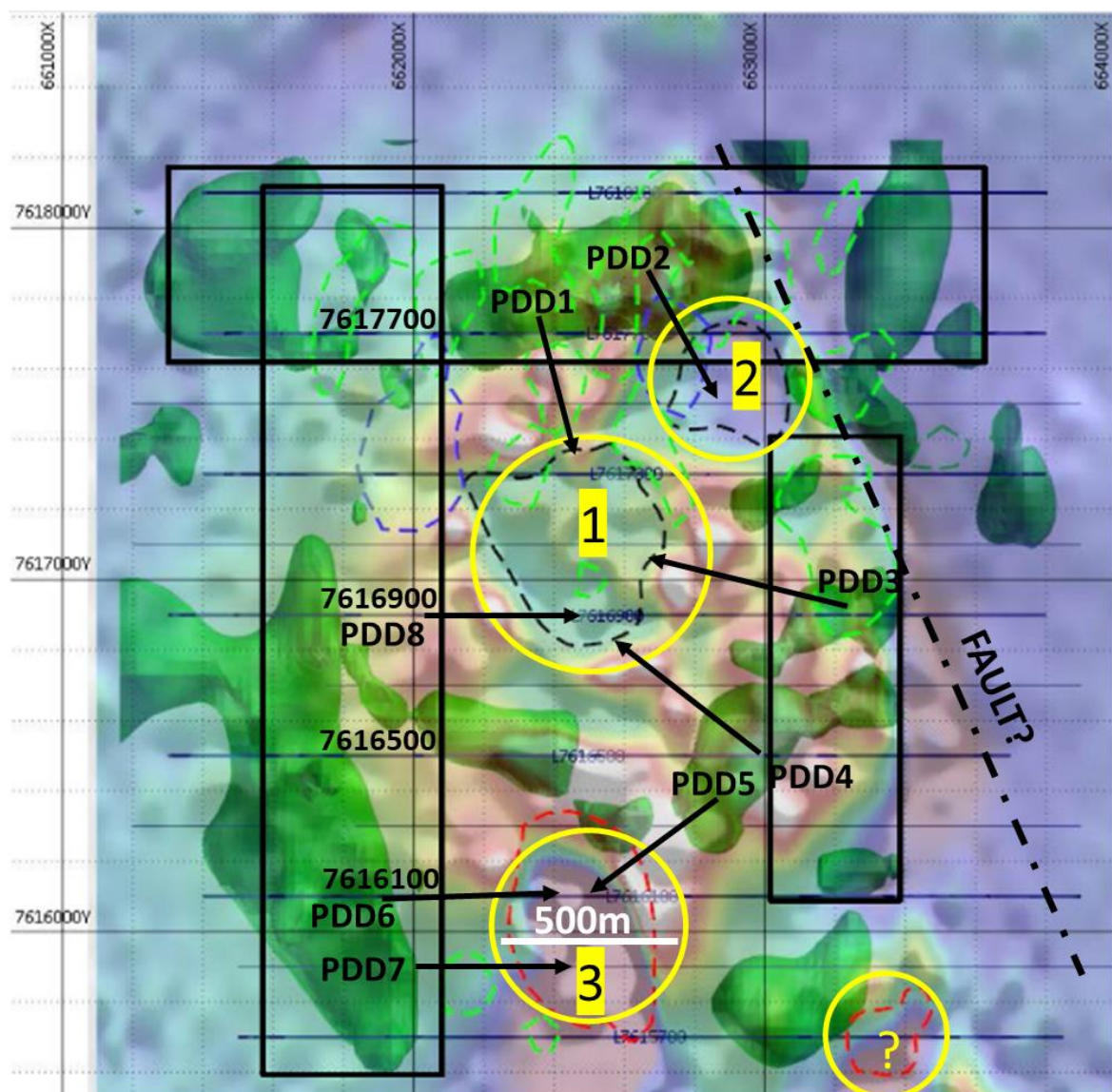
Figure 9: Shows location of proposed RC drillholes to test each of the interpreted porphyry targets. Exact hole locations will be confirmed in the field.
