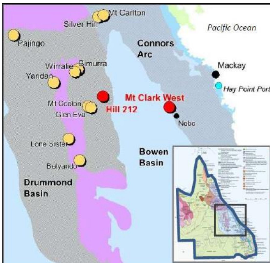
Figure 1 – Image shows the location of the Mount. Clark West (MCW) and Hill 212 tenements held by FEG. MCW is situated within Carboniferous volcanic rocks of the Connors Arc. Overlying Bowen Basin Permo-Triassic sediments occur to the west. The occurrence of significant epithermal Au-Ag deposits further west within the Drummond Basin are also shown.
