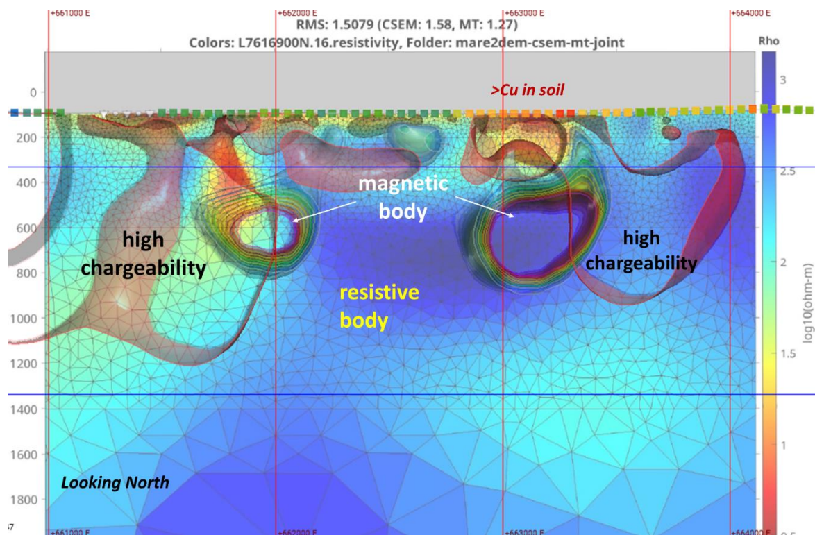
Figure 7: SGC interpreted resistivity image for MIMDAS survey line 7616900N. The image shows an envelope of low resistivity & high chargeability surrounding a central zone of high resistivity. The occurrence of high magnetic bodies immediately adjacent to the resistive zone are considered to be priority drill targets to test for porphyry type mineralization. The east-most area is coincident with a broad (1km) zone of high Cu in soil.
