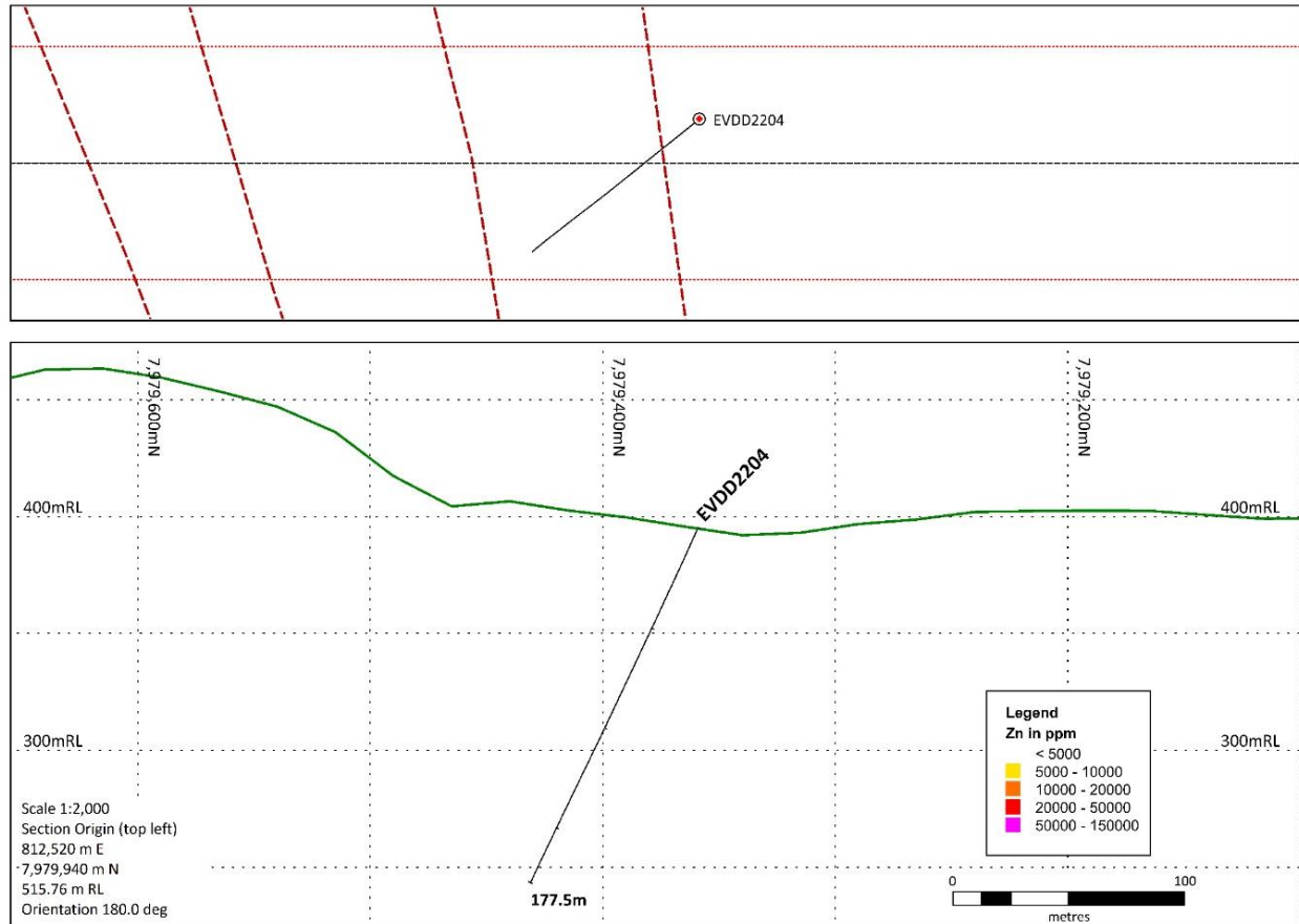
Figure 7: Cross Section 812520mE - EVDD2204
