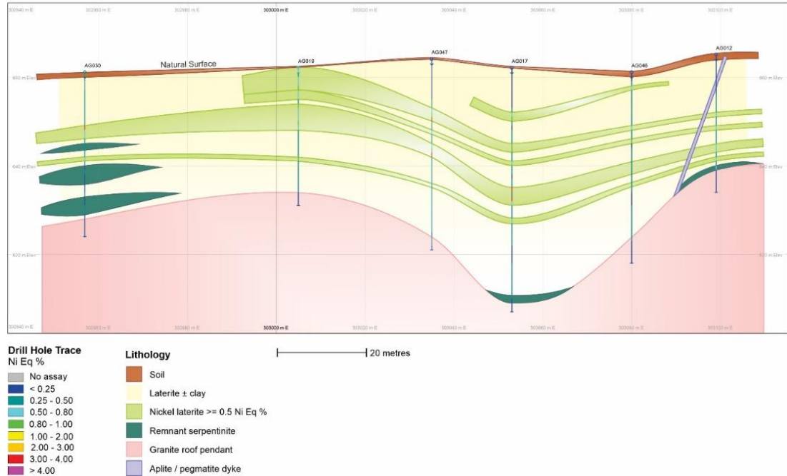
Gunnawarra Nickel Laterite Cross Section 8012050 mN
