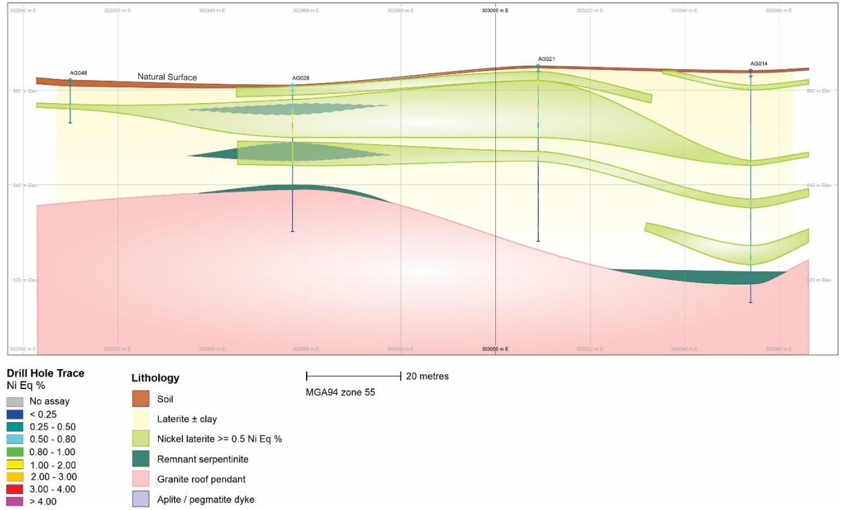
Figure 5 Gunnawarra Nickel Laterite Cross Section 8012100
