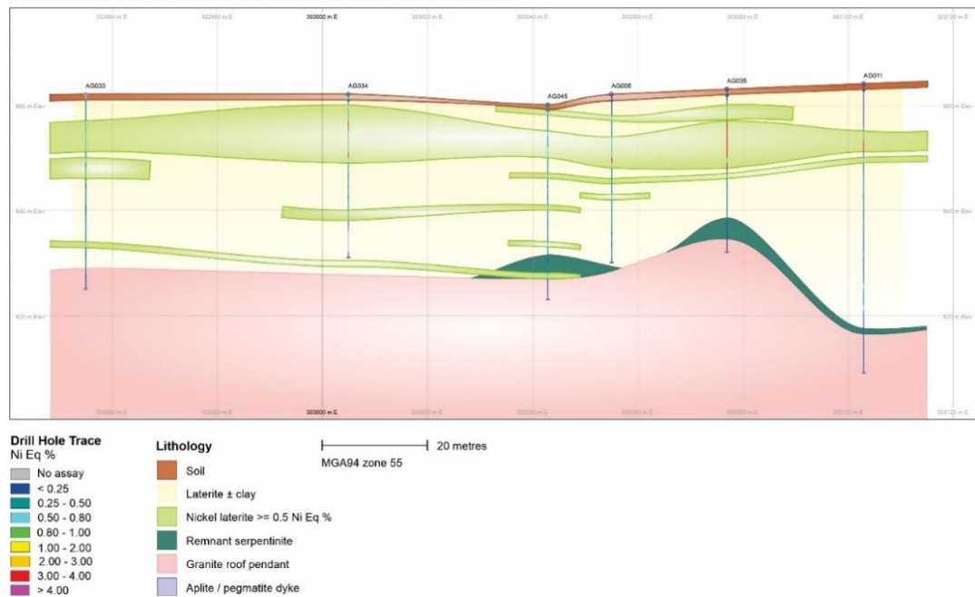
Gunnawarra Nickel Laterite Cross Section 8012000 mN
