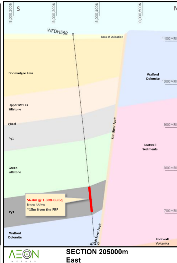
Figures 6 and 7: Cross sections through 205,655mE (showing relative location of WFDH561) and through 205,000mE (showing relative locations of WFDH558)
