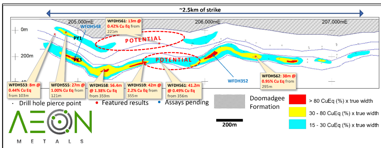
Figure 3: Schematic long section through the Amy zone at Walford Creek, showing the location of recent drill holes (as pierce points) and mineralisation intensity (CuEq Grade times True Width) 1 .
