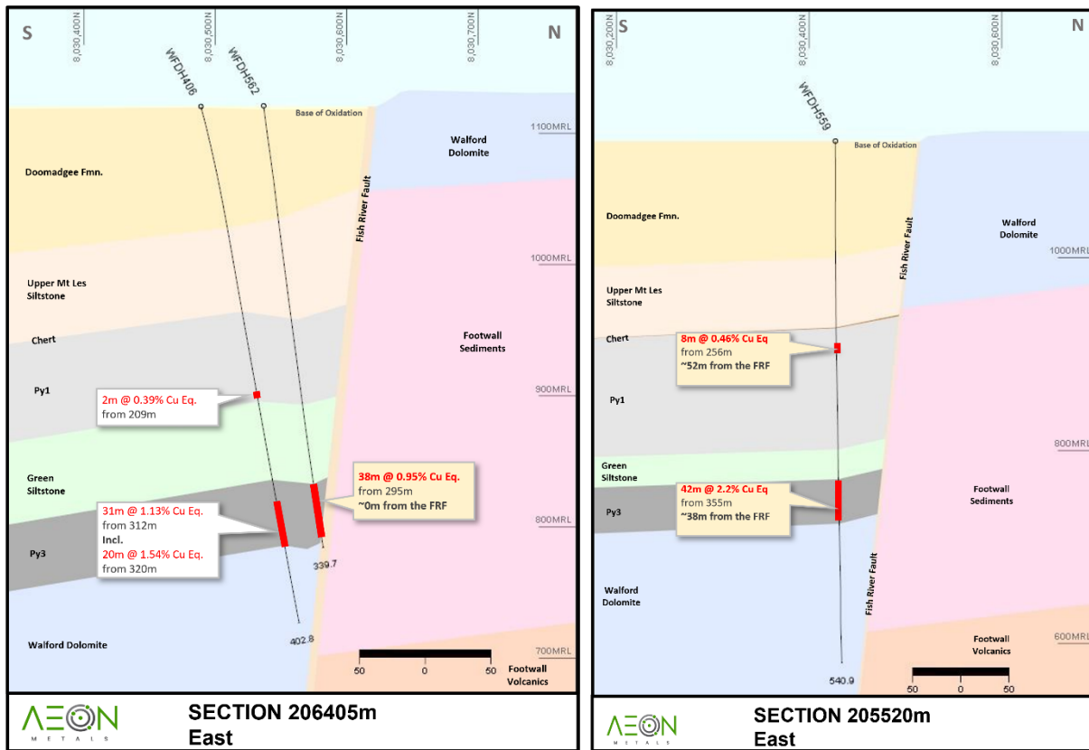
Figures 8 and 9: Cross sections through 206,405mE (showing relative location of WFDH562 and WFDH406) and through 205,520mE (showing relative locations of WFDH559)
