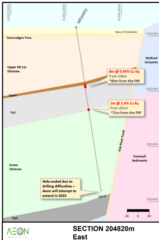
Figures 4 and 5: Cross sections through 204,820mE (showing relative location of WFDH553 and through 204,890mE (showing relative locations of WFDH555 and 378)
