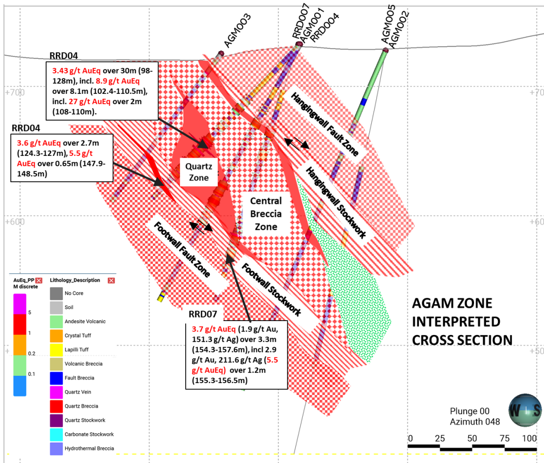
Figure 3: Interpretive cross section of the first completed drill section across the Agam Zone. The zone is characterised by hangingwall and footwall faults at zone boundary with outer quartz stock vein zones and central zone of massive quartz and quartz breccia. The best developed (and highest grade) mineralization occurs within the central breccia zone and zones of massive quartz contained therein. The cross section will be revised as more holes are drilled. Assays are pending for Phase 2 AGM drill holes.
