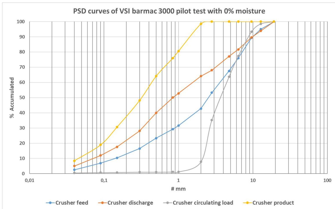
Figure 15: PSD curves of VSI barmac 3000 pilot test with 0% moisture.
