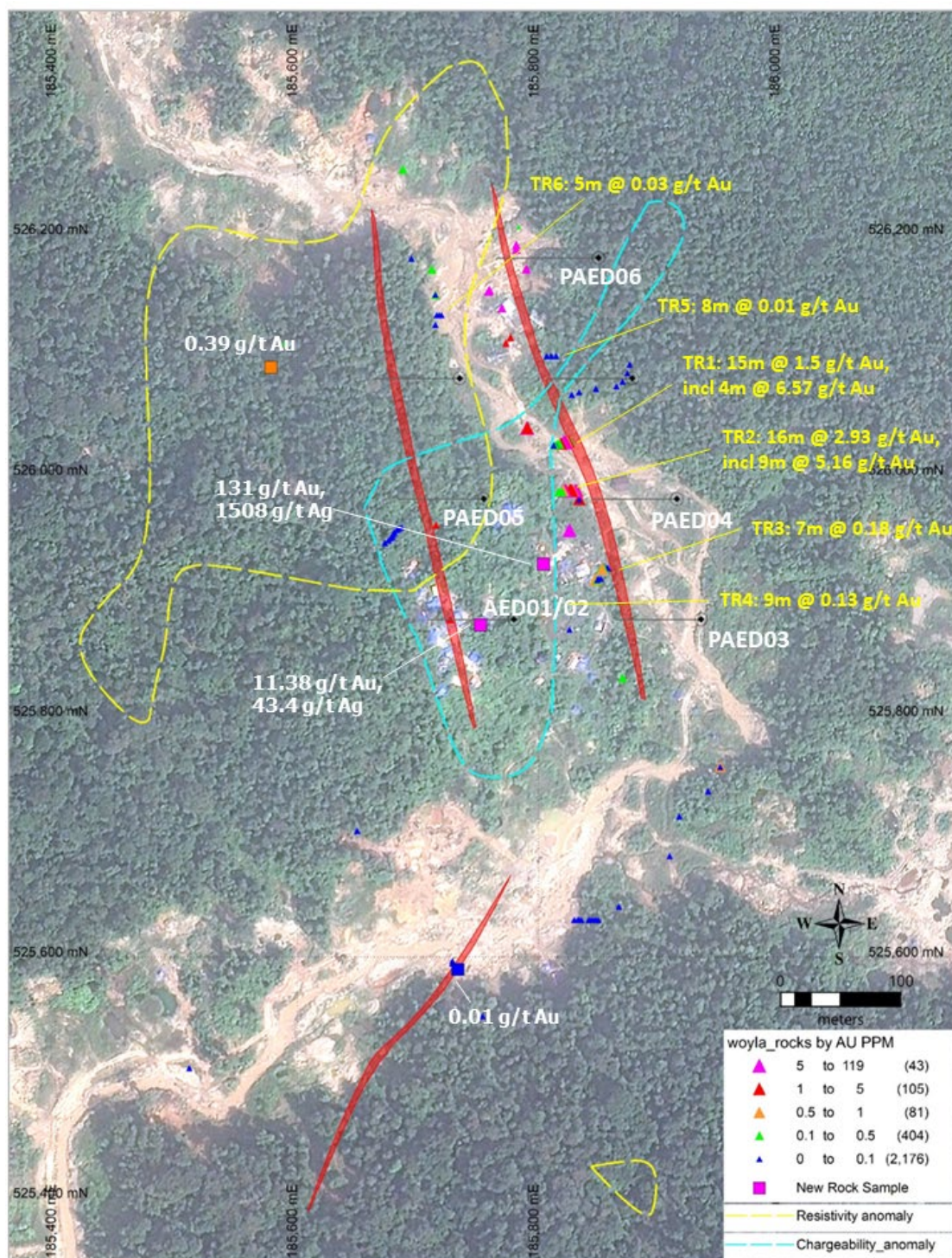
Figure 1: Plan map showing the interpreted extent and orientation of quartz veins within the Aloe Eumpeuk prospect area and distribution of historical and recent surface rock samples with assays. See Figure 2 and refer to ASX release of March 17, 2023 for additional sample assay information. The locations of current (AED) and planned drill holes (PAED) are indicated as are the surface extents of interpreted IP resistivity and chargeability anomalies. Refer to Figure 2 for highlighted rock samples. Historical trench (TR) locations and channel sample assay results are as reported by Barrick (1997). Trenches 5,6 had poor vein exposures due to thick alluvium cover.
