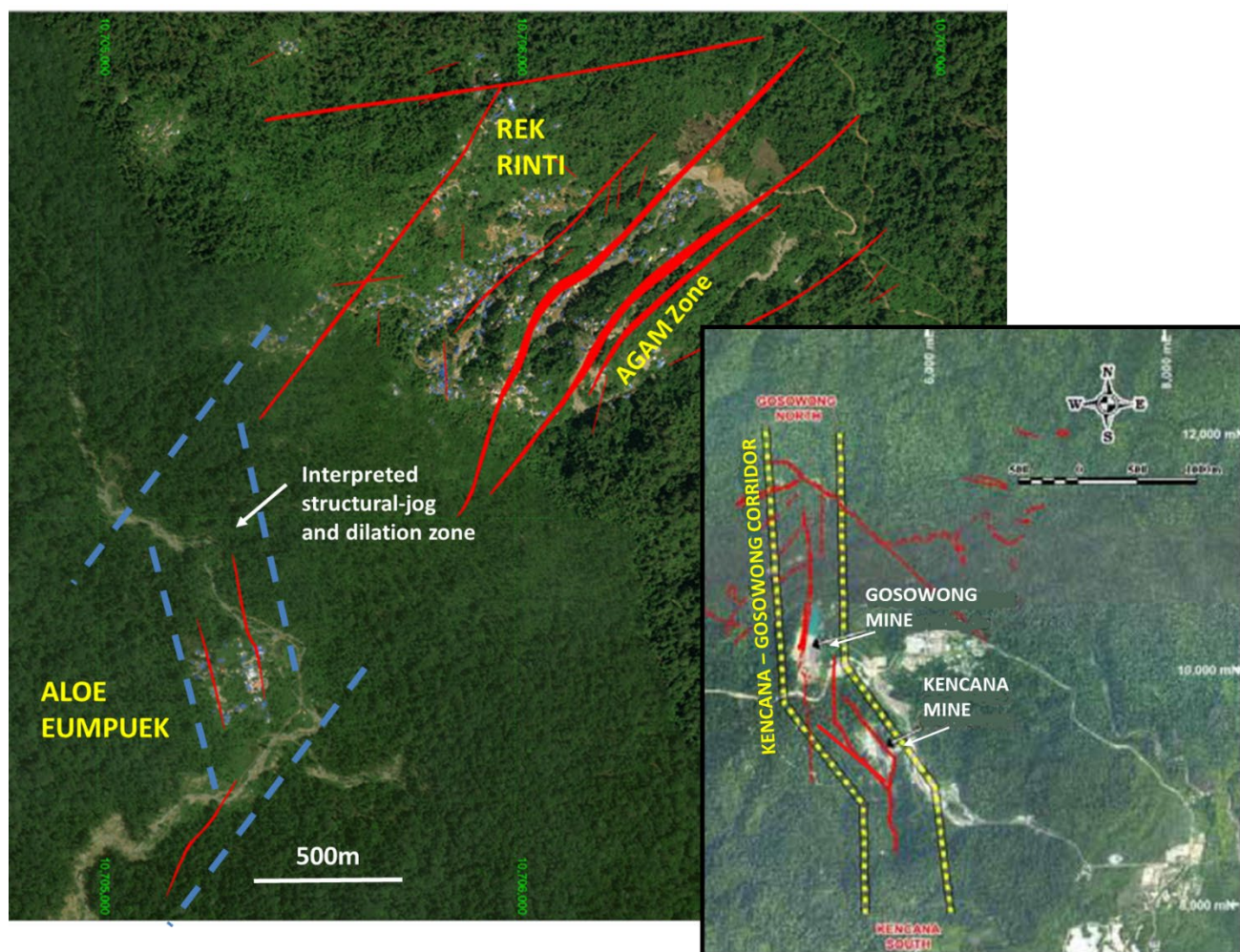
Figure 3: Image shows the location and interpreted structural setting of the Aloe Eumpeuk vein system. This is analogous to the structural setting of the Kencana gold deposit within the Gosowong gold district as shown in the inset map, modified from Technical Report of the Gosowong Property in North Maluku Province, Indonesia, December 31, 2011, Newcrest Mining.
