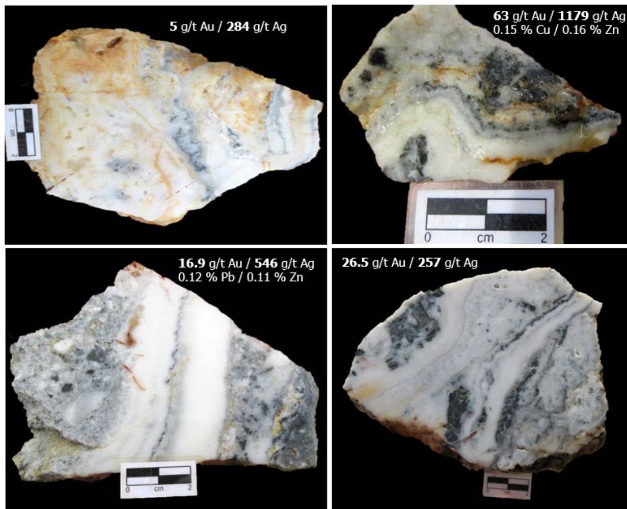
Figure 4: Photos of samples of Aloe Eumpeuk quartz vein material taken from artisanal miner pits. Samples show the presence of crustiform banded quartz with thin dark-grey ginguro band indicative of high-grade Au-Ag mineralization manifest as electrum and rare visible gold.
