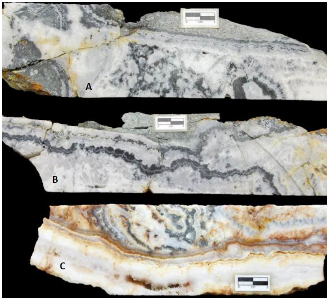
Figure 2: Above - Photos of samples of vein material taken from artisanal miner pits. Refer to Figure one for sample locations. Both samples show the presence of crustiform banded quartz with thin dark-grey ginguro bands containing the natural gold-silver alloy electrum and associated sulphide minerals. Below - Photos of drill core specimens from drillhole AED002 (see Figure 1) showing occurrence of dark-grey ginguro bands and fine-grain electrum and sulphide minerals within the ginguro (Figure 3). Photo A-75.7m, B-75.9m, C-78.6m
