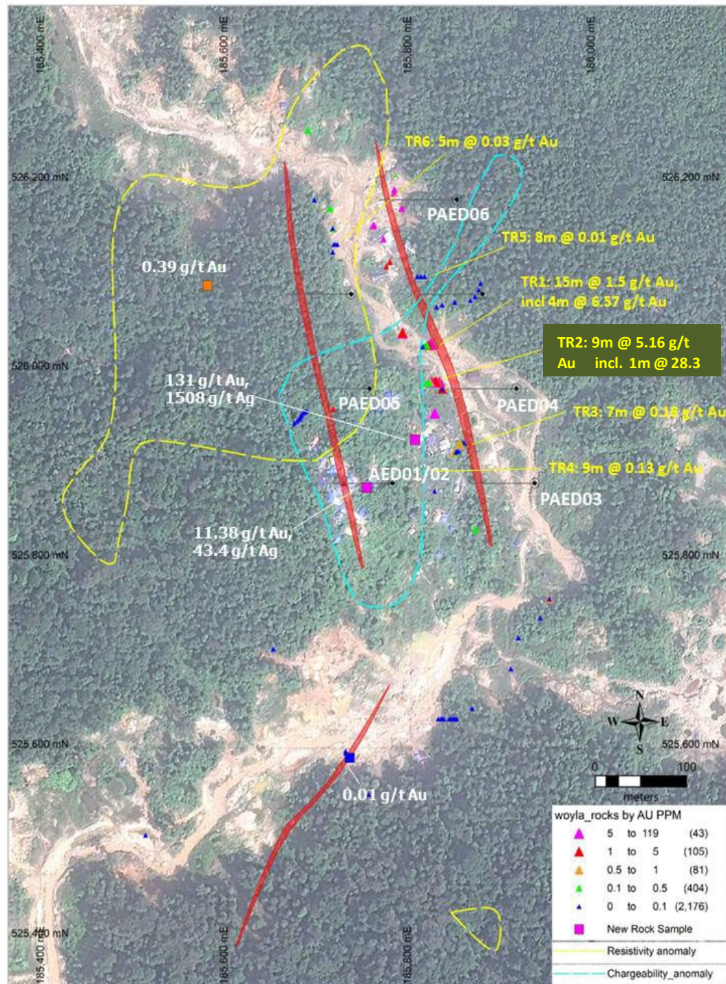
Figure 1: Plan map showing the interpreted extent of quartz veins within the Aloe Eumpeuk prospect area and distribution of historical and recent surface rock samples with assays. See Figure 2 and refer to ASX release of March 17, 2023 for additional sample assay information. The locations of current (AED) and planned drill holes (PAED) are indicated as are the surface extents of interpreted IP resistivity and chargeability anomalies. Refer to Figure 2 for highlighted rock samples. Historical trench (TR) locations and channel sample assay results are as reported by Barrick (1997). Trenches 5,6 had poor vein exposures due to thick alluvium cover.
