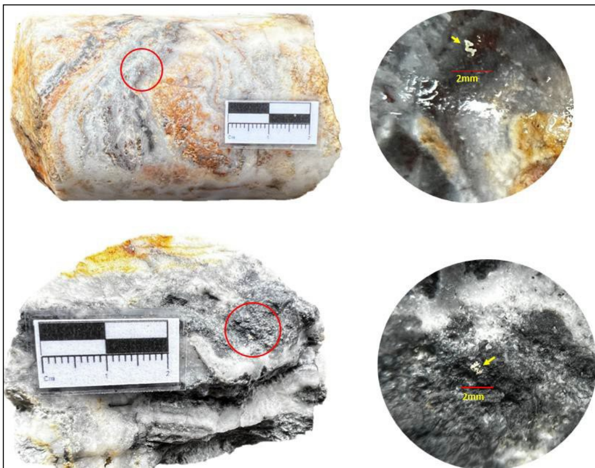
Figure 4: Photos of quartz veins with thin ginguro bands containing fine-grained specks of electrum and visible gold in AED002. TOP (75.5m), BOTTOM (76.1m).
