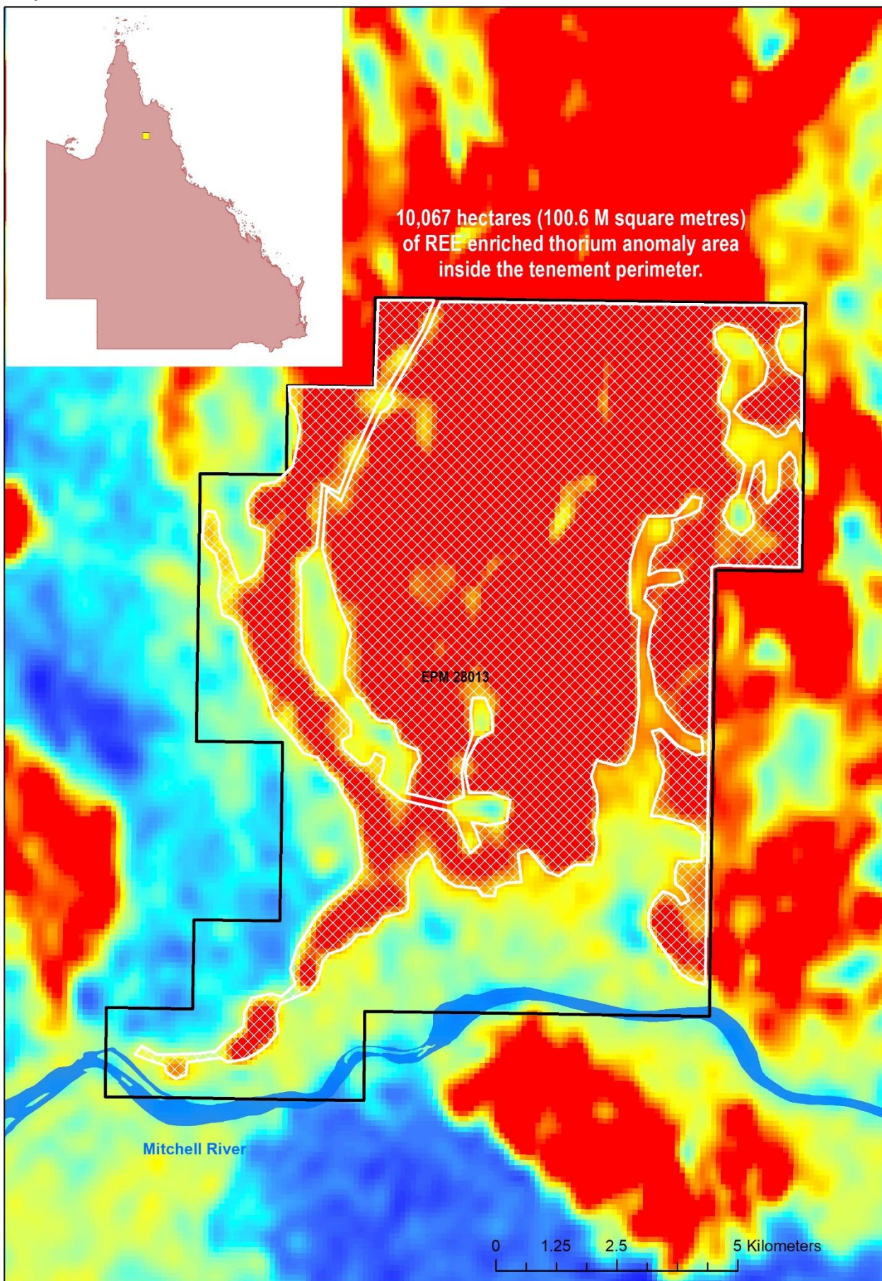
Figure 3: The size of the thorium anomaly correlating with REE enriched alluvial sands within the Project: tenement is
