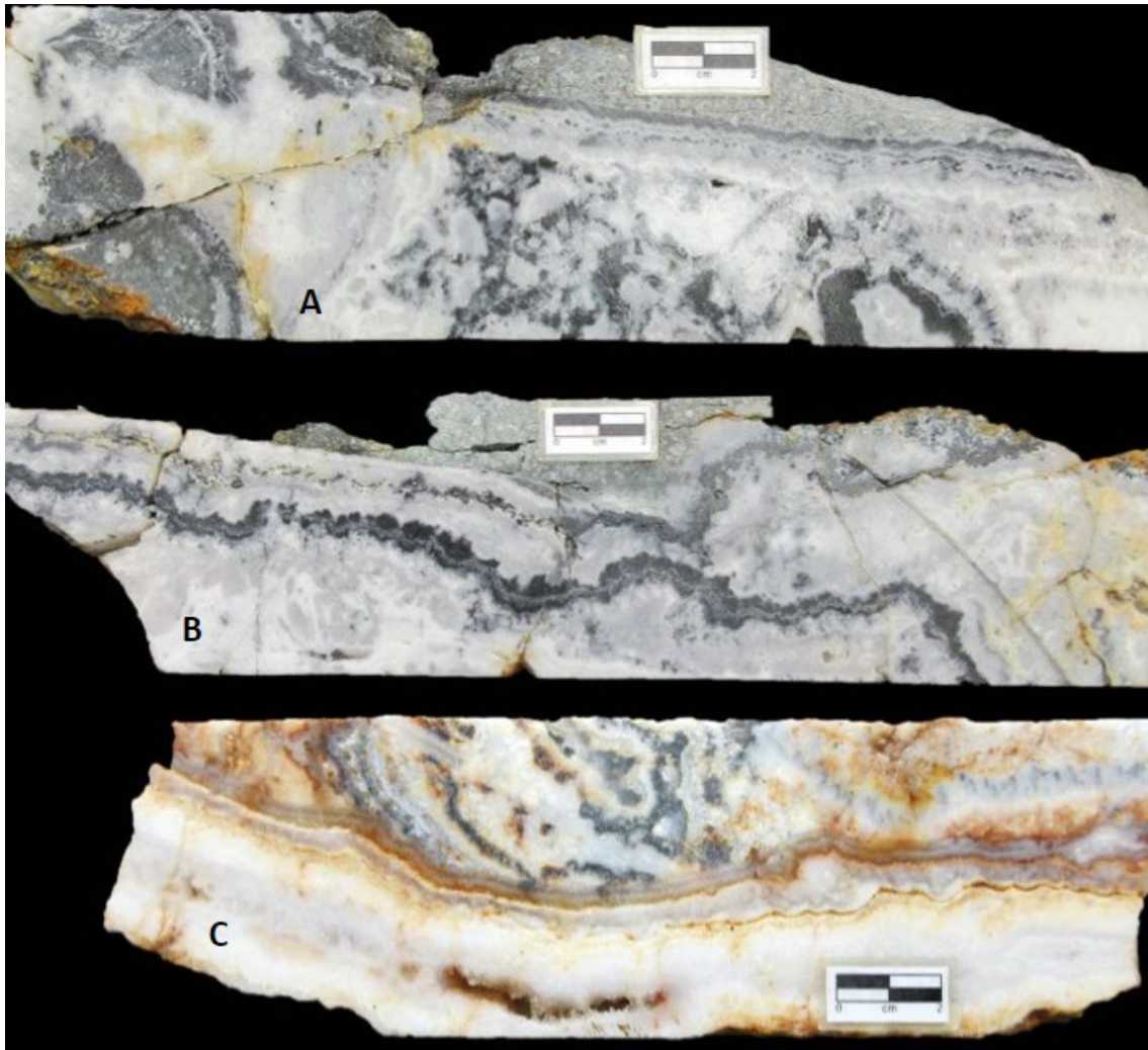
Figure 3: Photos of drill core specimens from drillhole AE02 (see Figure 1) showing occurrence of dark-grey ginkuro bands and fine-grain electrum and sulphide minerals within the ginkuro (Figure 4). Photo A-75.7m, B-75.9m, C-78.6m
