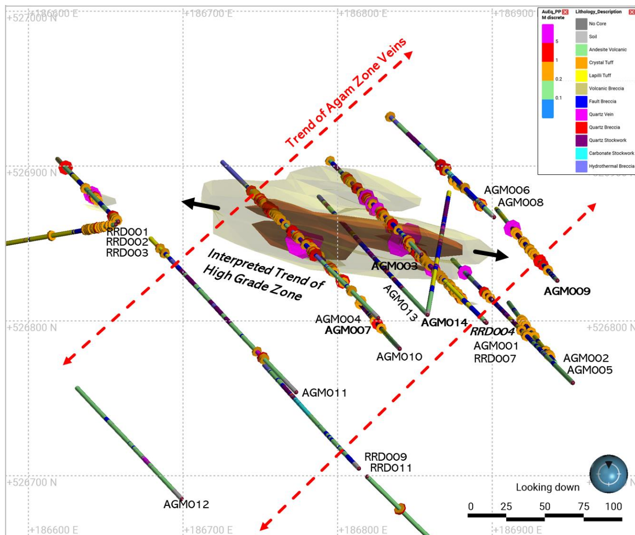
Figure 3: Plan map showing the interpreted surface extent of Agam Zone veins and the interpreted trend of the Agam high-grade Au-Ag zone. The high-grade zone may have developed within an oblique sigmoidal structural feature. The location of drillhole AGM014 is indicated as are other AGM holes completed as part of the current Phase 2 drill program. AGM holes are being drilled at 50m and 25m-spaced section to test the Agam zone continuity and also focus on discrete, structurally-controlled high grade shoots that occur within the vein/breccia zone. AGM014 is a 25m-spaced section to specifically target the high-grade Au-Ag zone intersected in RDD004.
