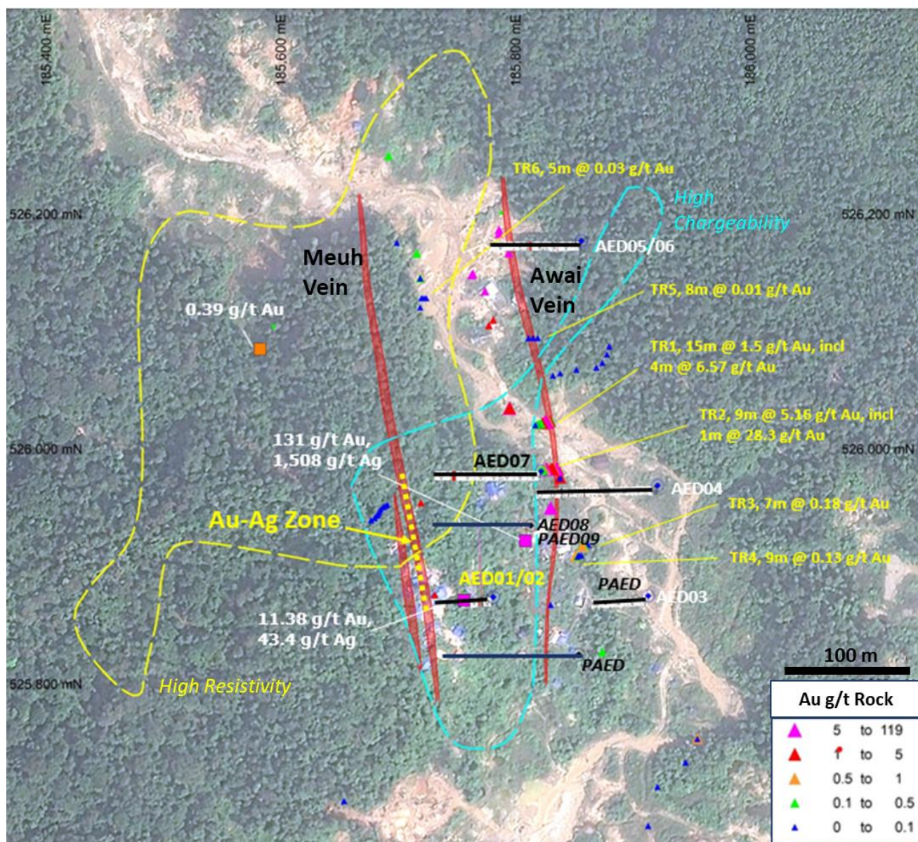
Figure 1: Plan map showing the interpreted surface extent of quartz veins within the Aloe Eumpeuk prospect area and distribution of historical and recent surface rock samples with assays. Refer to ASX release of March 17,2023 and April 17,2023 for additional sample assay information. The locations of current (AED) and planned drill holes (PAED) are indicated as are the surface extents of interpreted IP resistivity and chargeability anomalies. Historical trench (TR) locations and channel sample assay results are as reported by Barrick (1997). Trenches 5,6 had poor vein exposures due to thick alluvium cover. The inferred extent of a zone of visible gold/electrum associated with ginguro-bands in the Meuh vein is also shown.
