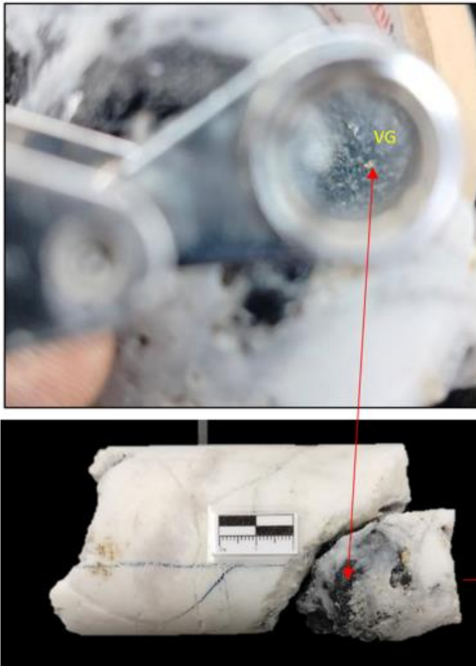
Figure 2: Section of quartz vein intersected at 109.1m in AED007. Fine-grained visible gold/electrum occurring within coarse clots of ginguero-hosted sulphide minerals.
