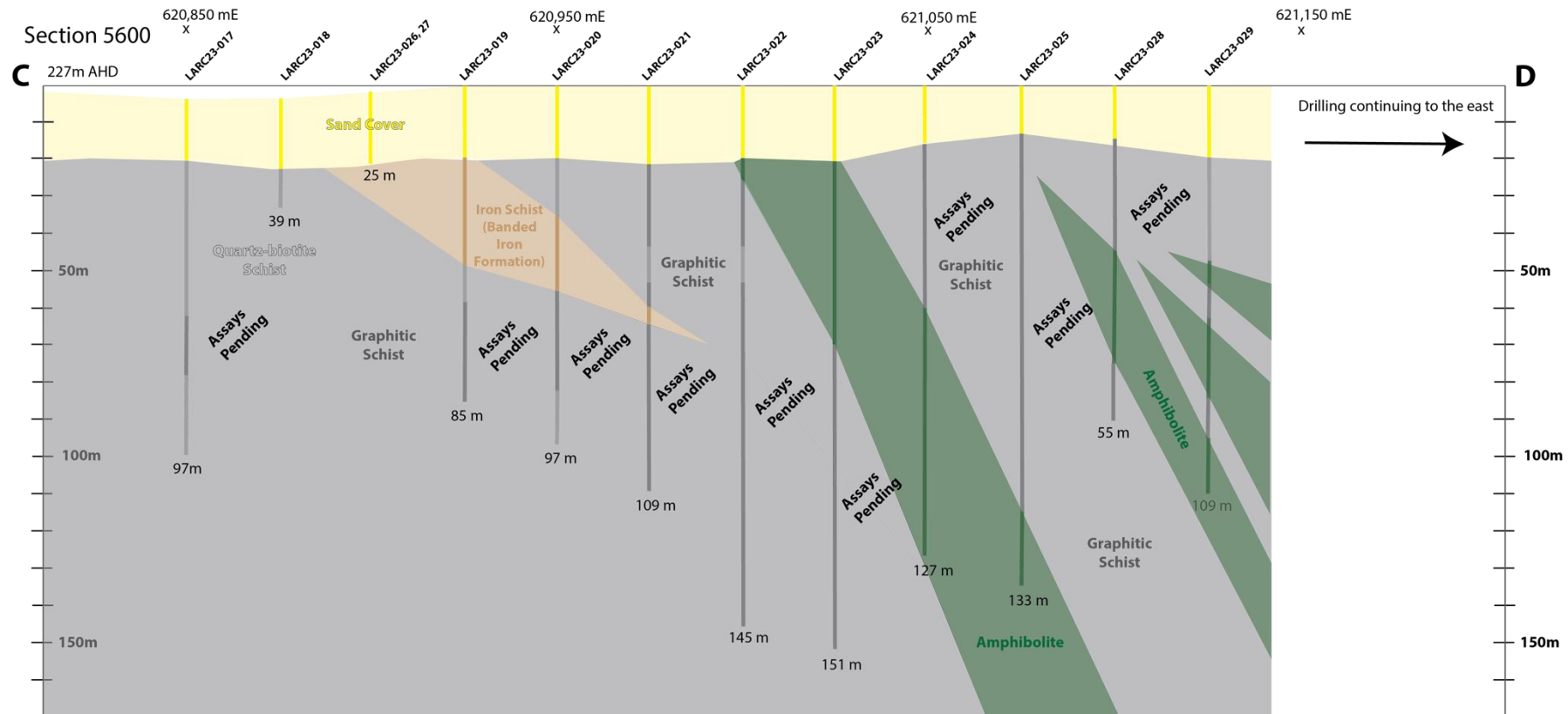
Figure 3. Traverse 2 - Section 5600, East-West section through the Lacroma Graphite Prospect – Scale 1:1
