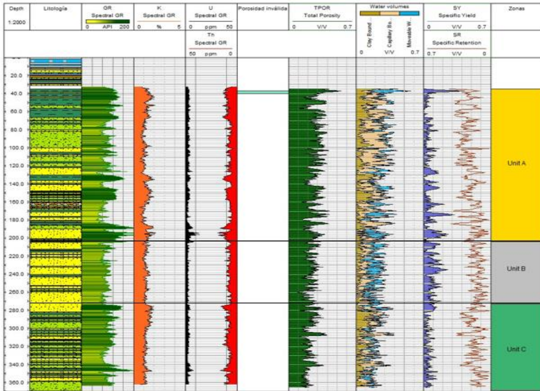
Figure 5: Geophysical log of hole K15R31, in the centre of the salar, showing Units A to C
