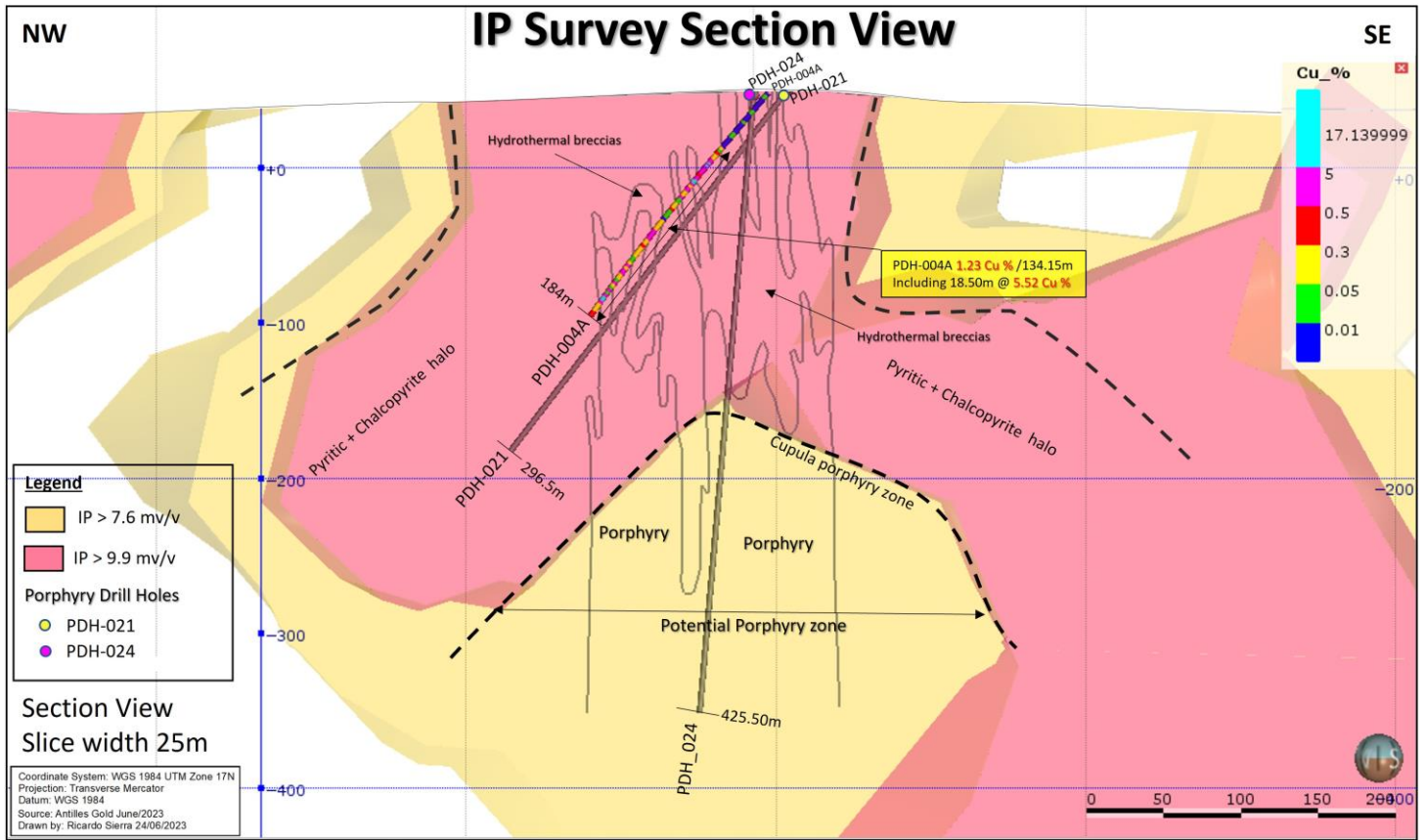
Induced Polarisation Survey Section 017 - Slice Width 25m
