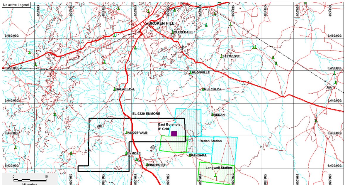
Figure 2: East Borehole Prospect Location within EL 9220 Enmore southeast of Broken Hill
