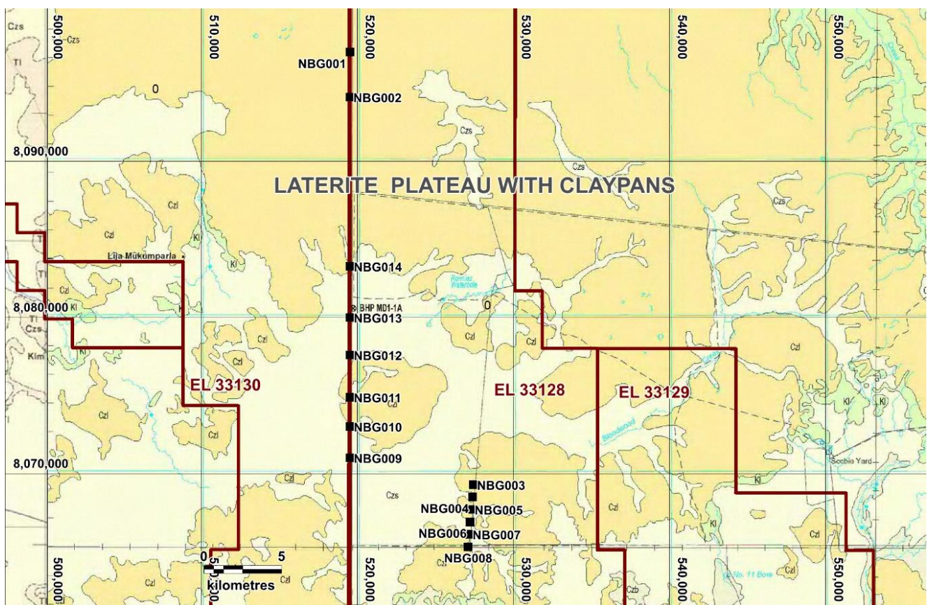
Figure 3 - Drill Locations on Geology (Wallhallow 250,000 Sheet)
