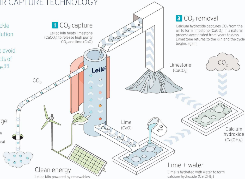
Caption: Heirloom’s Direct Air Capture process powered by Leilac’s renewably powered electric kiln.
