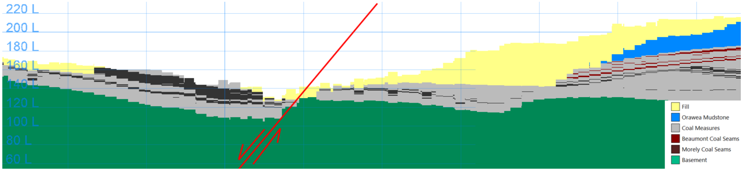
Figure 23: Section view through the deposit. The Black Diamond Fault and backfilled Coaldale East pit are shown
