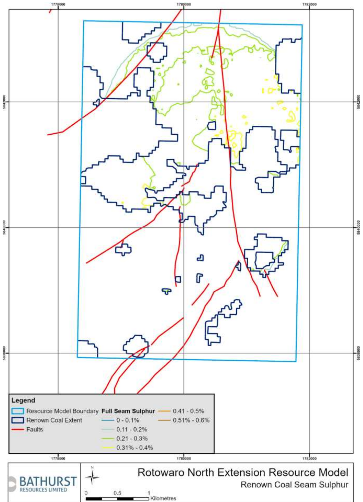
Figure 16: Plan showing the full seam sulphur isopachs of the RM coal seam
