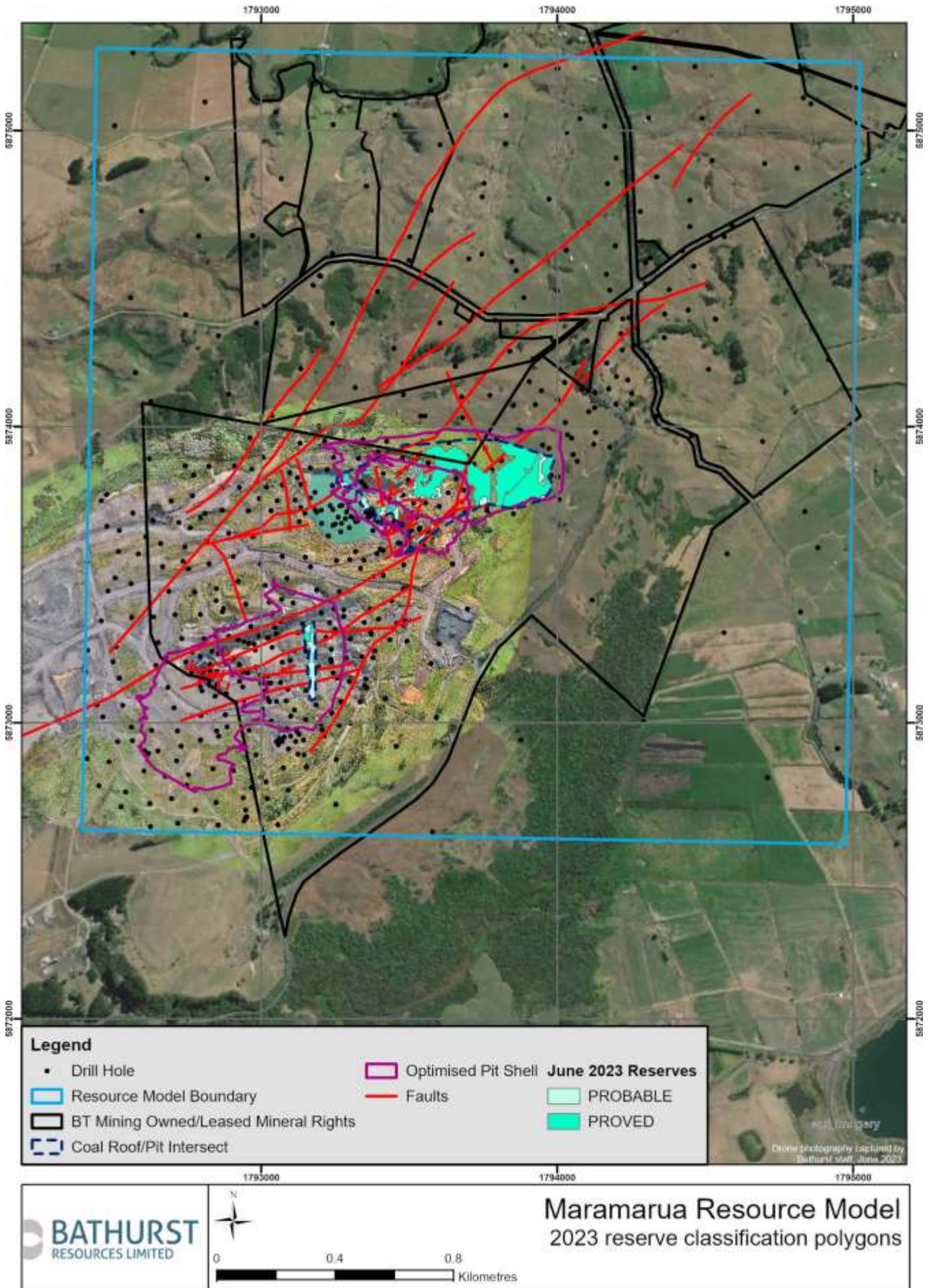
Figure 7: Maramarua reserve classification polygons with pit shell extents
