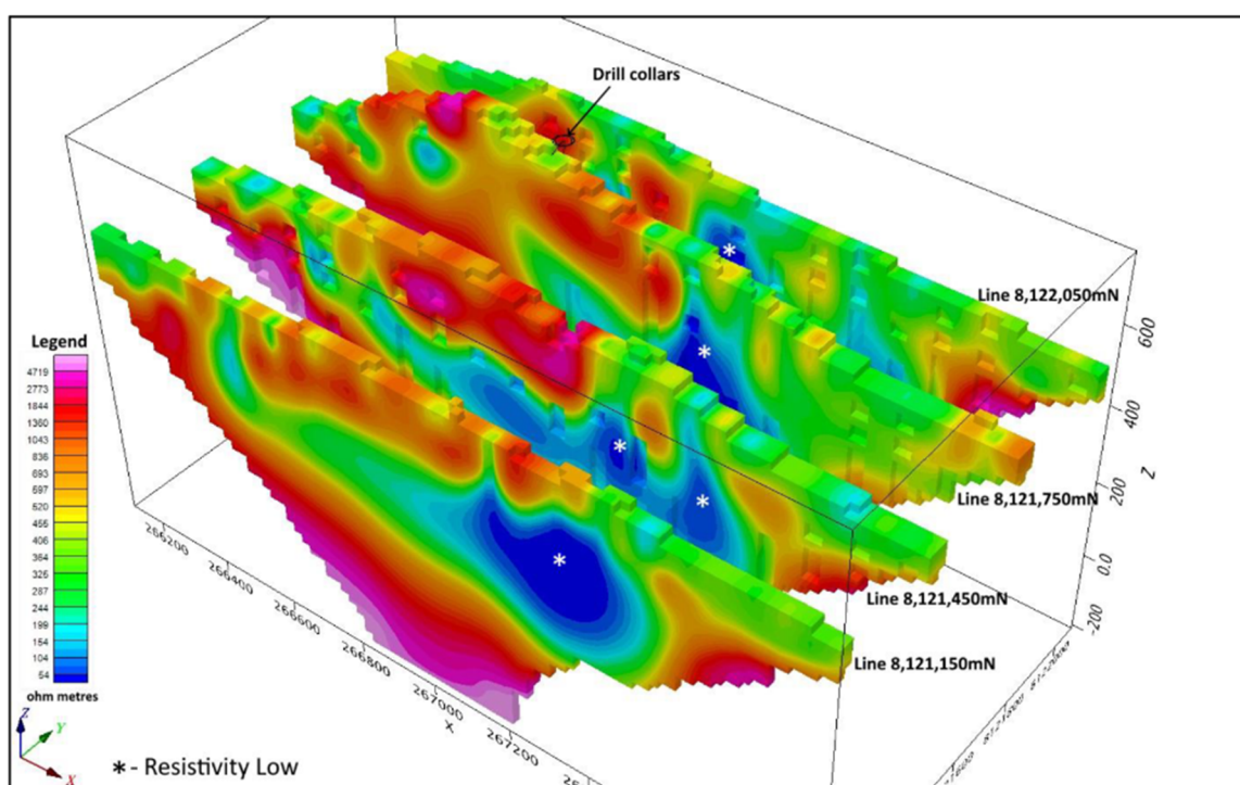
Figure 5. Maneater Hill Resistivity Sections
