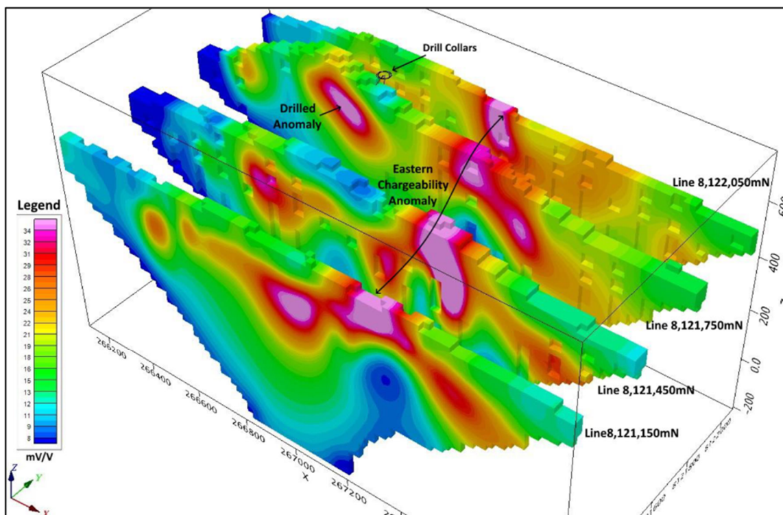
Figure 4. Maneater Hill Chargeability Sections
