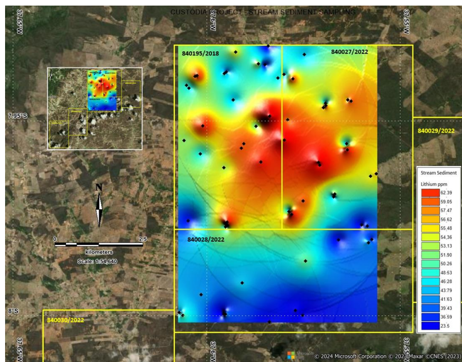
Figure 1. Thematic map of Anomalous Lithium values in stream sediment samples in Custodia tenements. Sample sites shown as black diamonds.
