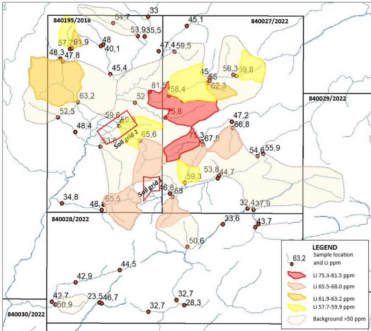
Figure 2. Custodia stream sediment sample anomalous catchments and the locations of previous soil grids in red polygons.
