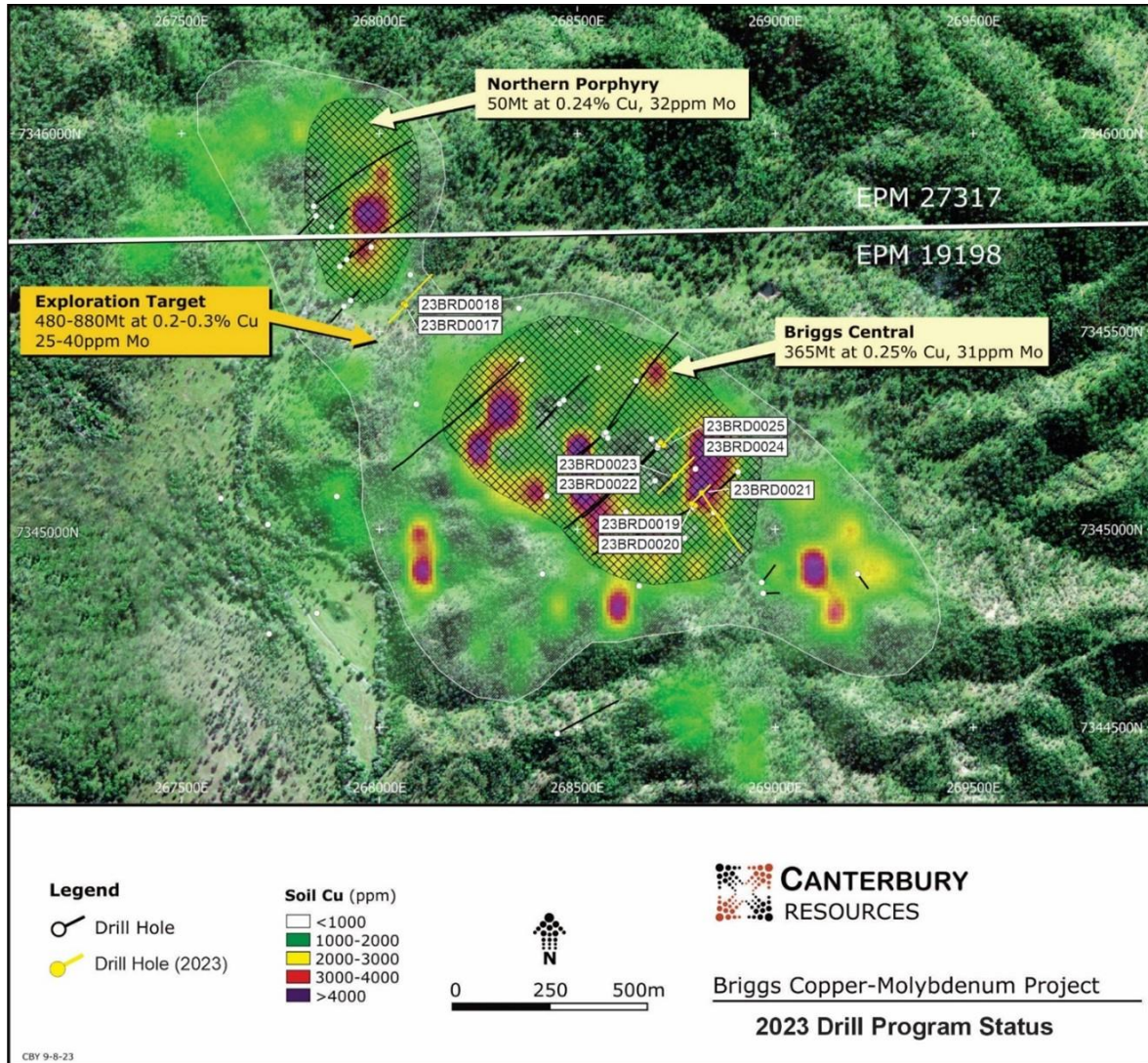
Figure 2 Plan displaying Cu in soil geochemistry, Exploration Target area outline based on 500ppm Cu contour (white) and existing Inferred Resource (hatched area), plus historic and recently completed drill holes.
