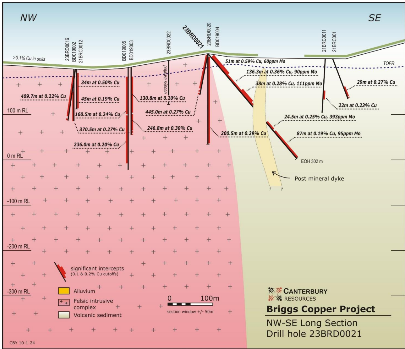
Figure 3 Long-Section for 23BRD0021, Briggs Central
