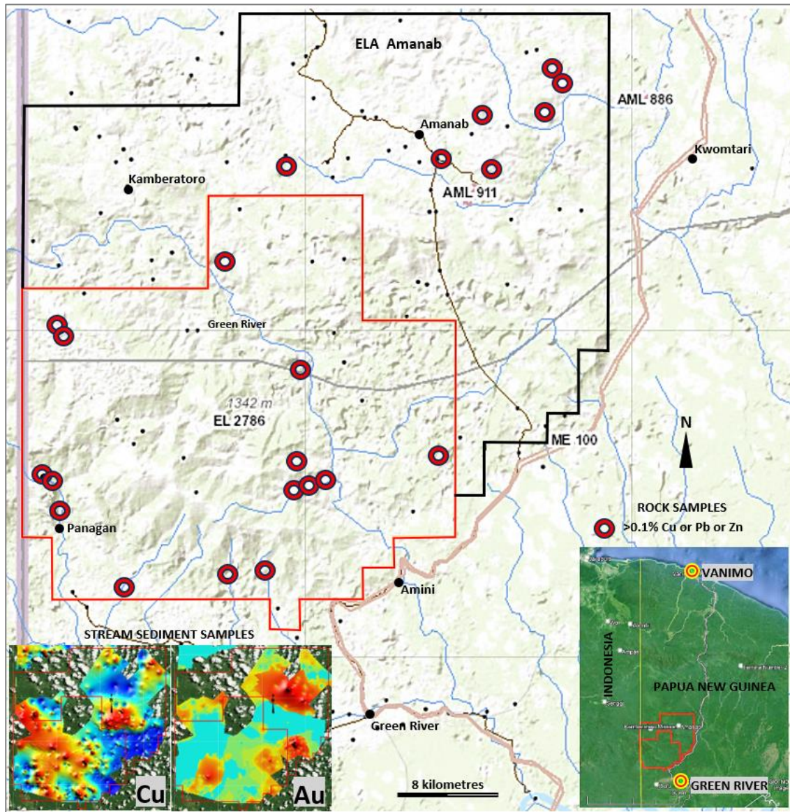
Figure 6. Location of the Green River and Amanab Ela's in West Sepik Province.
