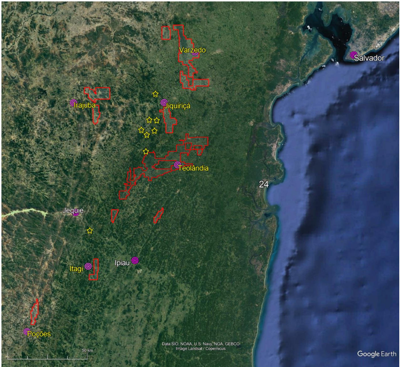
Figure 1. Location of the Jequié region REE and Niobium projects.
