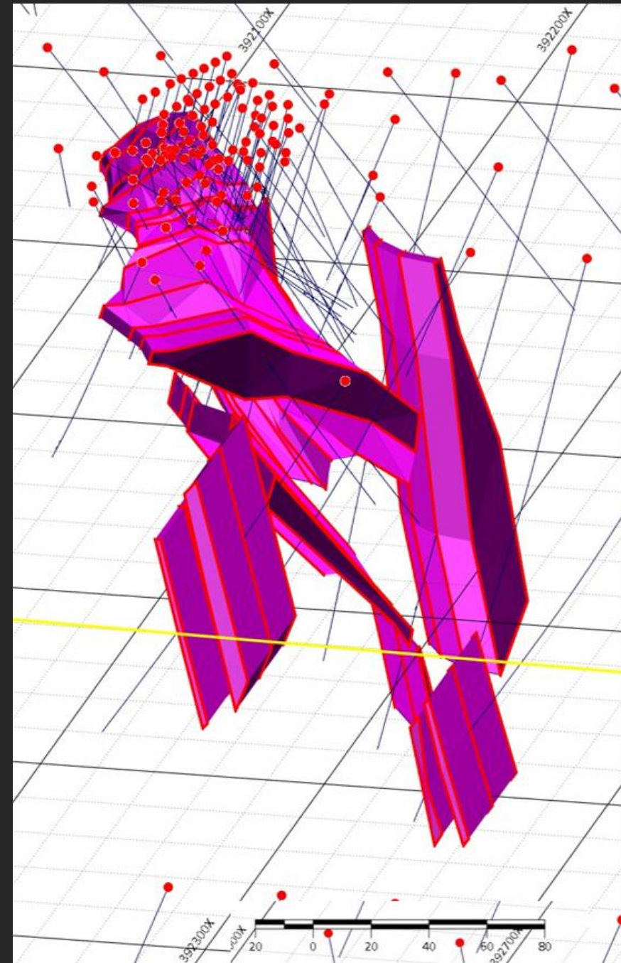
Garibaldi mineralised envelope looking north-west
