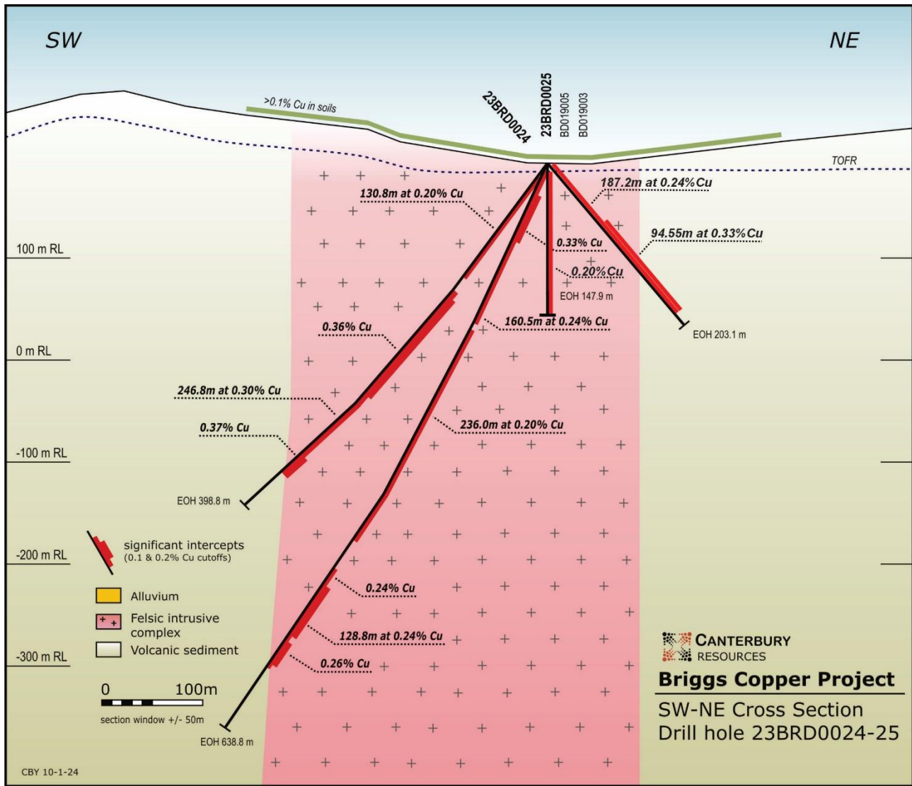
Figure 5 Cross-Section for 23BRD0024 & 23BRD0025, Briggs Central
