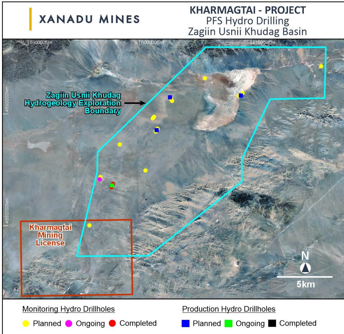
Figure 1. PFS Water Drilling in ZUK Basin
